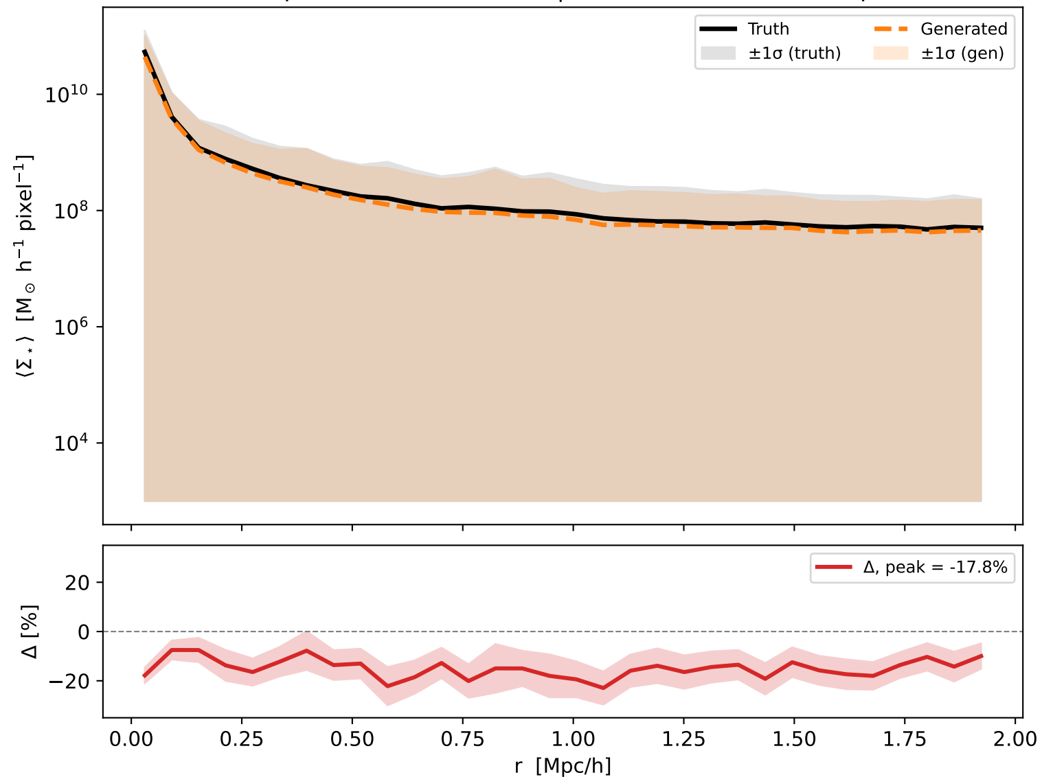
P7: BCG-centered radial profile — Stars channel Exact-peak halos (N=1733) | centered on truth BCG peak
