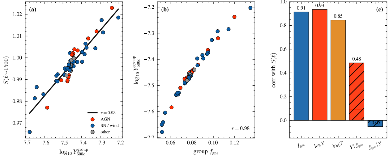
Figure 8: The Compton- Y bridge resolves the tightest single-quantity predictor of the field-level suppression. (a) S(\ell) (\ell \sim 1500) vs. \log_{10} Y_{500c}^{\text{group}} , r = 0.93 . (b) Y_{500c}^{\text{group}} vs. group f_{\text{gas}} , r = 0.98 — the two are nearly degenerate at fixed mass and redshift. (c) raw and partial correlations with S(\ell) : f_{\text{gas}} 0.91, \log Y 0.93, \log T 0.85, Y | f_{\text{gas}} (partial) 0.48, f_{\text{gas}} | Y (partial) \approx 0 — Y subsumes essentially all of the predictive power of f_{\text{gas}} alone.
