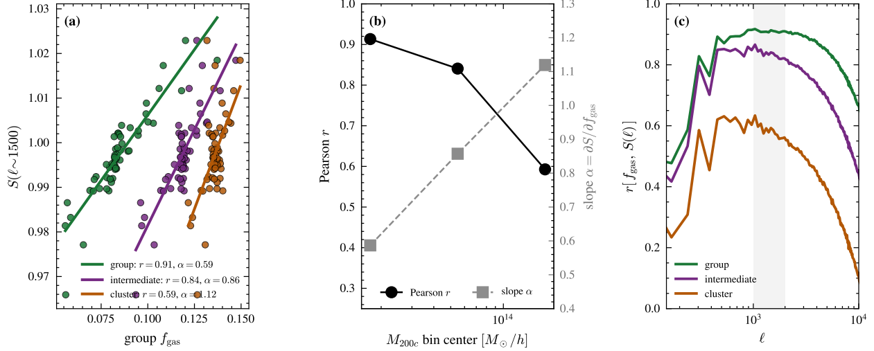
Figure 9: The bridge fit separately in three M_{200c} bins (group, intermediate, cluster). (a) S(\ell)(\ell \sim 1500) vs. group f_{\text{gas}} per mass bin. (b) Pearson r and best-fit slope \alpha = \partial S / \partial f_{\text{gas}} vs. mass-bin center. (c) r[f_{\text{gas}}, S(\ell)] vs. \ell per mass bin. The correlation loosens toward cluster scale even as the slope steepens, consistent with the group-dominated suppression signal discussed in the text.
