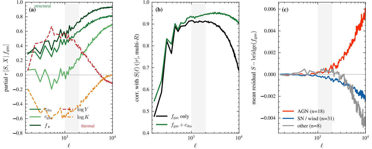
Figure 10: When and why the single-predictor bridge breaks down. (a) Partial correlation of each halo-level quantity with S(\ell) (at fixed f_{\text{gas}} ) vs. \ell : thermal quantities ( \log Y , \log K ) dominate below \ell \sim 1500 , structural quantities ( c_{\text{DM}} , c_{\text{gas}} , f_{\star} ) above. (b) The two-variable f_{\text{gas}} + c_{\text{DM}} bridge (green) restores the correlation with S(\ell) relative to the f_{\text{gas}} -only bridge (black), especially at high \ell . (c) The mean residual S - \text{bridge}(f_{\text{gas}}) by feedback family, showing AGN runs above and SN/wind runs below the bridge at high \ell . [TODO: this figure’s own family-classification legend (AGN n = 18 , SN/wind n = 31 , other n = 8 ) does not match the classification used in Figure 6 (AGN 20, SN/wind 25, other 12) for the apparently identical 57-run 1P design; we have not been able to reconcile which classification script is authoritative from the source material available, and flag this discrepancy explicitly rather than silently pick one.]
