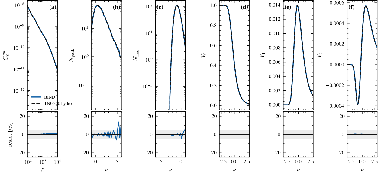
Figure 2: Field-level fiducial closure: BIND (solid) vs. TNG300 hydrodynamical truth (dashed) for the convergence power spectrum C_\ell^{KK} , peak counts N_{\text{peak}}(\nu) , minimum counts N_{\text{min}}(\nu) , and the three Minkowski functionals V_0, V_1, V_2(\nu) , with fractional residuals (shaded \pm band) in the lower row. C_\ell^{KK} and the Minkowski functionals agree to within a few percent across the full range shown; peak counts show larger ( \sim \pm 15\% ) but statistically consistent scatter in their sparsely populated high- \nu tail, while minimum counts stay within \sim \pm 7\% across their full range. This is the headline result of the paper: at fixed subgrid parameters, the BIND lightcone is statistically indistinguishable from the true hydrodynamical lightcone across the full non-Gaussian statistic set used by Stage-IV WL analyses.
