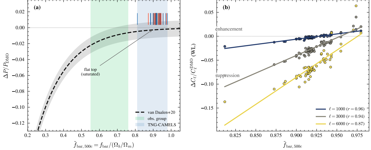
Figure 11: The TNG-CAMELS design samples only the saturated top of the global baryon-fraction–suppression relation. (a) \Delta P/P_{\text{DMO}} vs. the renormalized baryon fraction \tilde{f}_{\text{bar},500c} , van Daalen et al. functional form (van Daalen et al., 2020) (dashed), with the TNG-CAMELS 1P range (blue band, \tilde{f}_{\text{bar}} \approx 0.81\text{--}0.98 ) shown against the observationally preferred group-scale band (green). (b) the WL suppression relation \Delta C_\ell/C_\ell^{\text{DMO}} vs. \tilde{f}_{\text{bar},500c} at three multipoles, r = 0.96, 0.94, 0.87 at \ell = 1000, 3000, 6000 .
