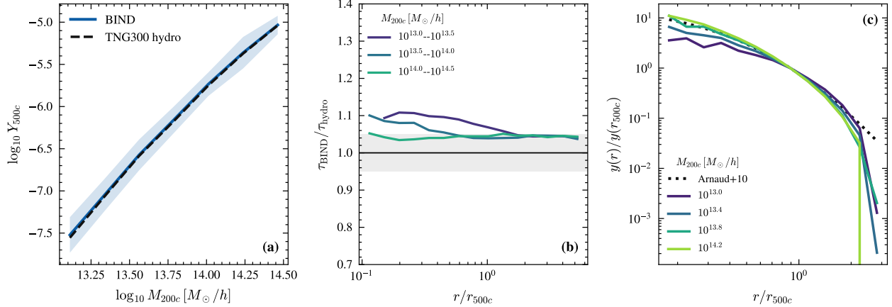
Figure 3: Halo-level thermodynamic closure at snapshot 96 ( z \approx 0.03 ). Left : the Y_{500c} – M_{200c} relation, BIND (solid) vs. TNG300 hydrodynamical truth (dashed), with 1\sigma intrinsic-scatter bands overlapping across 10^{13} – 10^{14.5} M_{\odot}/h . Middle : the stacked electron-column ratio \tau_{\text{BIND}}/\tau_{\text{hydro}} by mass bin, \sim 1.05 – 1.15 at group scale and closer to unity at the highest mass bin shown. Right : projected pressure profiles y(r)/y(r_{500c}) in four mass bins compared to the Arnaud et al. universal profile (Arnaud et al., 2010), matching to \sim 2 r_{500c} .
