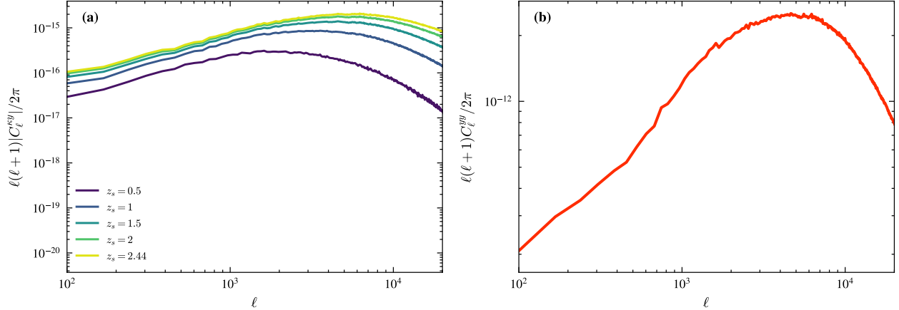
Figure 4: Tomographic cross- and auto-power spectra at fiducial parameters. Left : \ell(\ell+1)|C_\ell^{ky}|/2\pi for all five source-redshift bins, z_s = 0.5, 1.0, 1.5, 2.0, 2.44 . Right : the tSZ auto-spectrum \ell(\ell+1)C_\ell^{yy}/2\pi . Both spectra are computed with the ray-traced (deflected-ray) y -plane, not a Born-approximation slab sum (Section 2.2).
