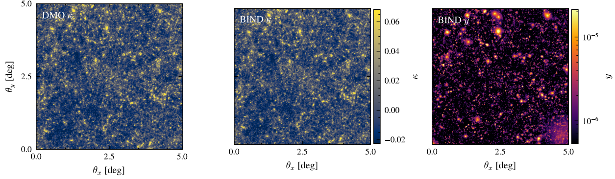
Figure 1: Fiducial BIND lightcone maps over the full 5 \times 5 \text{ deg}^2 field of view. Left : the paired DMO-only convergence at identical geometry, used as the common-mode reference for all suppression ratios in this paper. Middle : BIND convergence \kappa at source redshift z_s = 1.0 , sharing the color scale with the left panel. Right : the BIND Compton- y map from the same realization. The painted field is visually distinct from the DMO progenitor as an overall smoothing of the field-wide small-scale texture (most apparent in the diffuse, non-halo regions) rather than a localized change at individual peaks, and the y map traces halo cores with compact, feedback-sculpted morphology — the qualitative signature the quantitative validation in Figure 2 confirms statistically.
