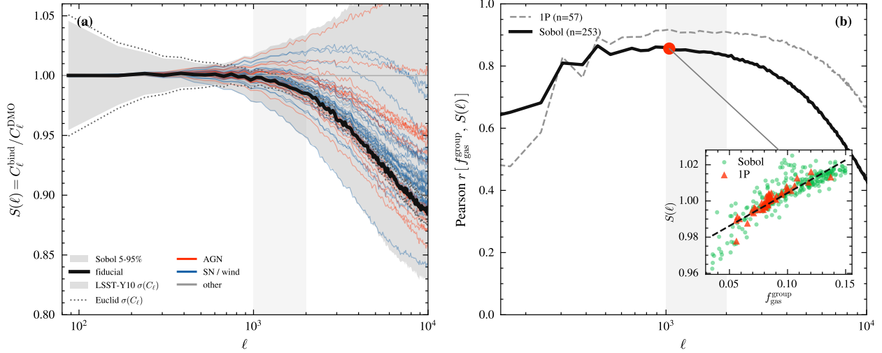
Figure 12: The bridge is robust from the 1P corners to the full Sobol design. Left: S(\ell) envelopes for the fiducial run, the 1P design ( n = 57 ), and the Sobol design ( n = 253 ), with LSST-Y10 and Euclid shape-noise bands for reference. Right: Pearson correlation r[f_{\text{gas}}^{\text{group}}, S(\ell)] vs. \ell for both designs, peaking at r \approx 0.86 – 0.91 near \ell \sim 1000 – 1500 ; inset shows the Sobol scatter at \ell = 1037 ( r = 0.86 ).
