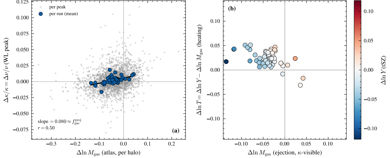
Figure 5: The per-halo \rightarrow per-peak bridge, 1P feedback suite. Left : WL peak height excursion \Delta\kappa/\kappa vs. the per-halo gas-mass excursion \Delta \ln M_{\text{gas}} ; grey points are individual peaks, blue points are per-run means. The best-fit slope, 0.080, matches the projected gas fraction of these halos; the per-peak correlation is r = 0.50 , while the run-averaged relation is clean. Right : the ejection–heating plane, \Delta \ln M_{\text{gas}} (ejection, what \kappa probes) vs. \Delta \ln T (heating, the residual y probes beyond mass loss), colored by \Delta \ln Y (the total tSZ observable). This is the map-level realization of the R(\nu) = f_{\text{gas}} \cdot T decomposition of Section 3.2.
