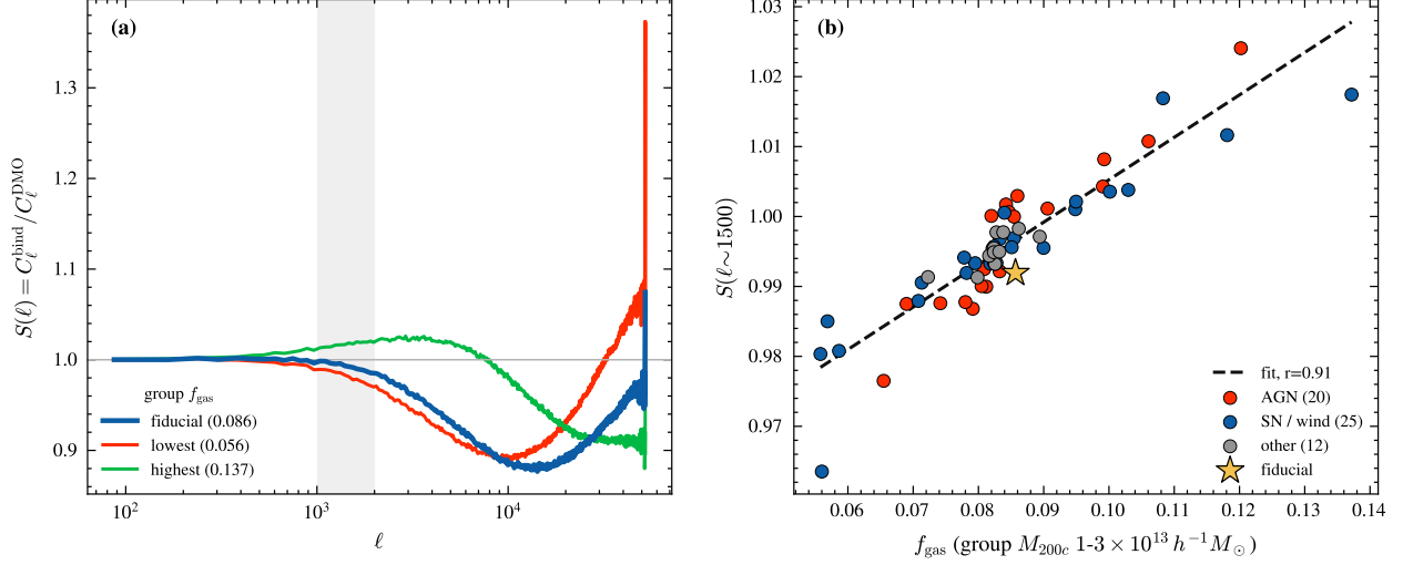
Figure 6: The group-scale, van-Daalen-style bridge. Left : S(\ell) suppression curves for the fiducial, lowest- f_{\text{gas}} , and highest- f_{\text{gas}} 1P runs, showing the CIC-aliasing upturn at \ell \gtrsim 2 \times 10^4 discussed in Section 4. Right : S(\ell)(\ell \sim 1500) vs. background-subtracted group gas fraction ( M_{200c} = 1-3 \times 10^{13} M_{\odot}/h , R_{500c} ) for 57 feedback-varied lightcones, colored by feedback family (AGN, SN/wind, other). The correlation is r = 0.91 . This is the direct analog, at the field level, of the van Daalen baryon-fraction-suppression relation (van Daalen et al., 2020).
