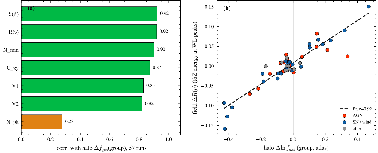
Figure 7: The bridge generalizes across the statistic set. Left : absolute correlation of each field-level statistic with the group-scale \Delta f_{\text{gas}} across the 57-run 1P suite: S(\ell) 0.92, R(\nu) 0.92, N_{\text{min}} 0.90, C_{\text{ky}} 0.87, V_1 0.83, V_2 0.82, and N_{\text{pk}} 0.28 (shot-noise dominated). Right : the R(\nu) -vs.- f_{\text{gas}} scatter underlying the R(\nu) bar above, r = 0.92 .
