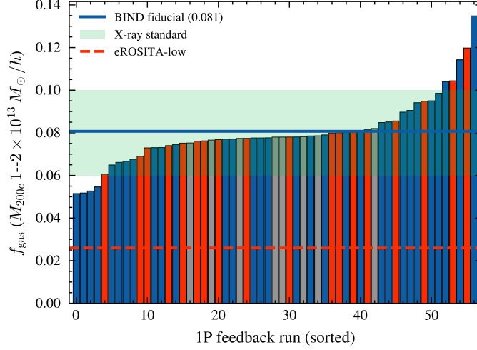
Figure 13: The corrected eROSITA gas-fraction tension. Sorted group-scale ( M_{200c} = 1-2 \times 10^{13} M_{\odot}/h ) f_{\text{gas}} across the 1P feedback suite, against the X-ray-standard band (0.06–0.10) and the eROSITA-low value (0.026; Popesso et al., 2026 ). The BIND fiducial value (0.081) sits within the X-ray-standard band; the minimum single-knob excursion (0.051) closes roughly half the gap to the X-ray band but does not reach eROSITA-low. This figure supersedes an earlier, LOS-contaminated “41% of cosmic” saturation claim (see Section 4).
