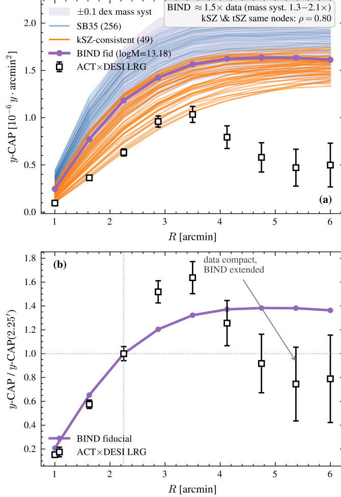
Figure 7: (a) y -CAP amplitude for all 256 Sobol nodes (light blue), the 49 kSZ-CAP-consistent nodes (orange), and the BIND fiducial run (purple) at the corrected DESI-LRG lensing mass \log M_{200c} = 13.18 M_{\odot}/h (Sailer et al., 2024), against the ACT \times DESI LRG data; the shaded band (purple) shows the \pm 0.1 -dex host-mass systematic alone, which spans 1.35\text{--}2.05 \times and dominates the visual spread (the in-panel annotation rounds this to one decimal, 1.3\text{--}2.1 \times ). (b) The y -CAP shape, normalized at 2.25' : BIND is more radially extended than the data (peak at 4.75' versus 3.5' ). Takeaway: the tSZ amplitude comparison is mass-selection-dominated – at the corrected mass, the kSZ and tSZ legs agree at the strong-feedback edge of the response, reversing the earlier (bug-driven) claim of an inter-probe tension.
