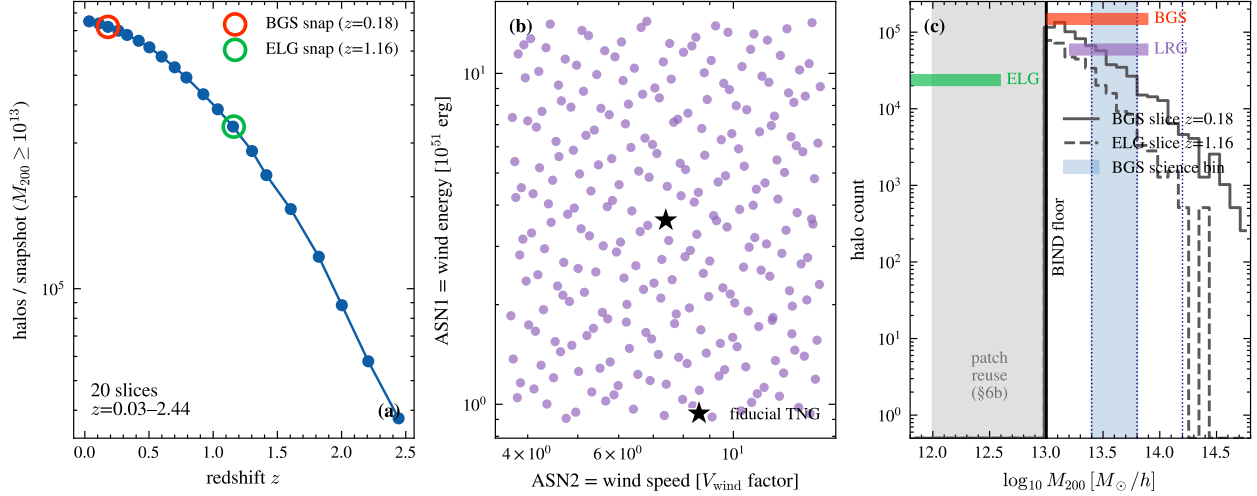
Figure 1: (a) Number of M_{200c} \geq 10^{13} M_{\odot}/h halos per lightcone snapshot slice across the 20 snapshots spanning z = 0.034 – 2.444 , with the BGS ( z = 0.18 ) and ELG ( z = 1.16 ) confrontation slices marked. (b) The 256-node Sobol feedback design in the physical units of its two dominant wind parameters (wind energy, wind speed factor), with the fiducial IllustrisTNG point starred. (c) The halo mass function at the BGS and ELG slices relative to the BIND painted-halo mass floor of M_{200c} = 10^{13} M_{\odot}/h and the DESI BGS/LRG/ELG host-mass bands; the shaded region below the floor is recovered only via the patch-reuse technique (Section 4.1). Takeaway: the design spans the full 30-parameter feedback prior on an identical halo population across the full observable lightcone.
