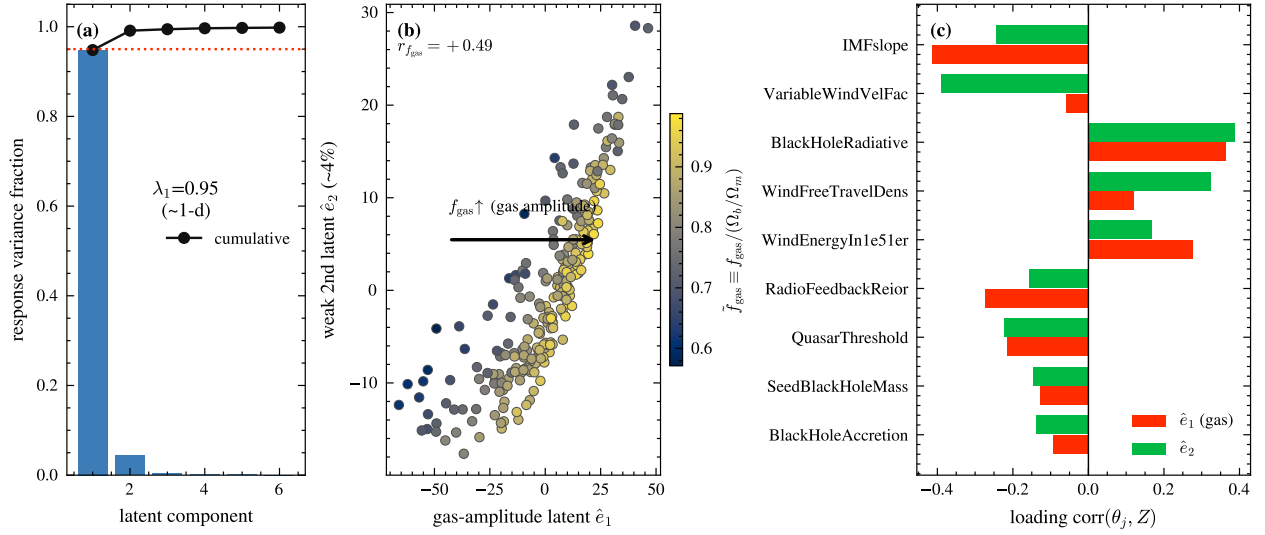
Figure 9: (a) Scree plot of the field-level ( S(\ell), C_\ell^{\kappa y} ) feedback response: component 1 already exceeds the 95%-variance line at \lambda_1 \approx 0.95 , with component 2 essentially flat. (b) The dominant gas-amplitude latent versus the (weak) second latent, colored by f_{\text{gas}} . (c) Parameter loadings on the two field-level axes. Takeaway: once projected through the lensing/tSZ kernel, the clean 2-D inner/outer-gas manifold of Figure 8 collapses to a single dominant gas-ejection direction.
