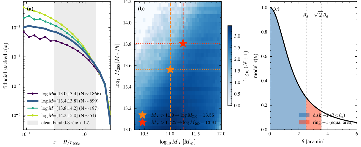
Figure 2: (a) Fiducial stacked \tau(R/r_{200c}) profile in four mass bins, with the “clean” fit band 0.3 < x < 1.5 shaded. (b) The stellar-to-halo-mass relation used to place the two DESI BGS M_{\star} cuts ( \log M_{\star} > 11.0, 11.25 ) onto host \log M_{200c} = 13.56, 13.81 respectively (the independent per-node mass estimate used for the Section 3.3 CAP-ratio confrontation gives the consistent \log M_{200c} = 13.60, 13.82 ; the \sim 0.01 – 0.04 dex difference reflects two separate SHMR-based reductions of the same M_{\star} cuts, not a physical discrepancy). (c) The compensated-aperture-photometry (CAP) filter: a disk of radius \theta_d (+1) minus an equal-area ring out to \sqrt{2}\theta_d (−1), applied identically to the painted \tau and y maps and to the DESI×ACT data. Takeaway: this is the exact filter and exact host-mass matching used for every data confrontation in Section 3.3.
