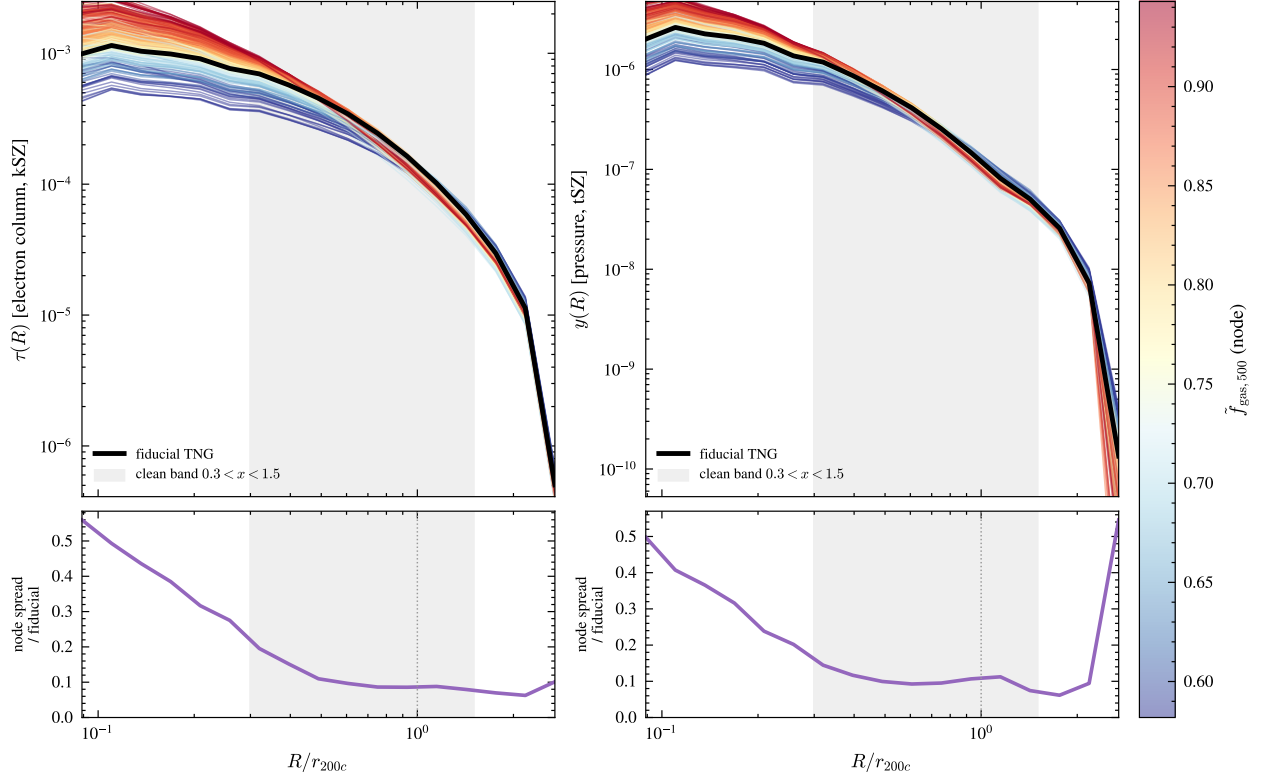
Figure 4: Stacked \tau(R) (left) and y(R) (right) profiles for all 256 Sobol feedback nodes in the BGS host mass bin ( \log M_{200c} \in [13.4, 13.8] , z = 0.18 ), colored by each node’s gas fraction \tilde{f}_{\text{gas},500} ; the fiducial TNG profile is overlaid in black. Bottom row: the ratio of the node-to-node spread to the fiducial profile as a function of radius, showing the feedback response is core-dominated. Takeaway: feedback reshapes both the \tau and y profiles smoothly and coherently with \tilde{f}_{\text{gas}} , most strongly at small radius.
