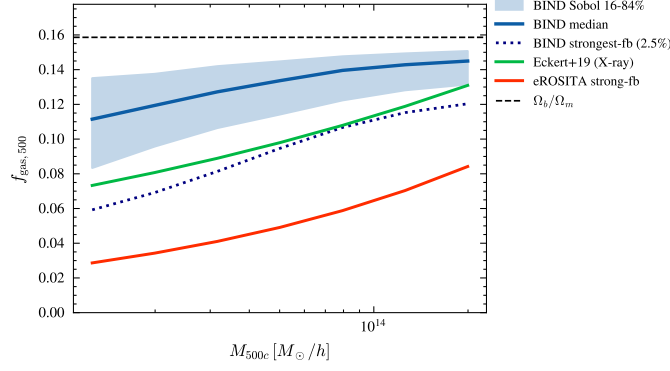
Figure 3: Gas fraction within 500c versus halo mass, for the 16–84% band, median, and strongest-feedback (2.5%) edge of the 256-node Sobol design, compared to the mainstream X-ray relation of Eckert et al. (2019) and the eROSITA strong-feedback edge of Popesso et al. (2024) , over M_{500c} = 10^{13} - 3 \times 10^{14} M_{\odot}/h . The horizontal dashed line marks the cosmic baryon fraction \Omega_b/\Omega_m . Takeaway: no point in the 30-dimensional TNG-like feedback prior – including its most extreme feedback tail – reaches the eROSITA band; the entire Sobol volume sits above the strong-feedback curve.
