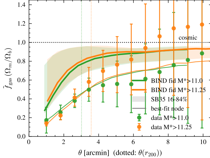
Figure 5: The \sigma_v -free, M_\star -matched CAP-ratio gas fraction \tilde{f}_{\text{gas}}(\theta) (Section 2.5) for the BIND fiducial run at the two DESI M_\star cuts (green, orange), the 256-node Sobol 16–84% band, and the best-fitting single node (legend rounds its fit to \chi^2 \approx 0 ; the precise value is \chi^2 \approx 0.1 , Section 3.3), against the real DESI×ACT data points with errors. The dotted vertical lines mark \theta(r_{200}) for each cut. Takeaway: the fiducial run is systematically above the data at small and intermediate aperture but roughly 20% of the Sobol design is statistically consistent with the data within its errors – this is the paper’s corrected, final kSZ-amplitude statement, superseding all earlier (cumulative-aperture) CAP numbers.
