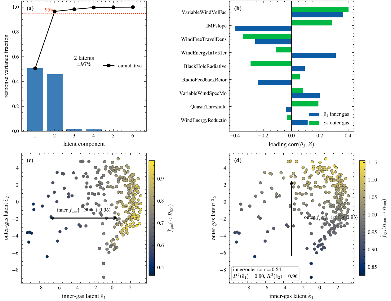
Figure 8: (a) Scree plot of the 30-parameter (\tau, y) feedback response: two components explain 97% of the variance. (b) Parameter loadings on the two latent axes, dominated by VariableWindVelFactor, IMFslope, WindFreeTravelDensFac, and WindEnergyIn1e51erg. (c,d) The same 2-D latent plane colored by inner-gas f_{\text{gas}}(< M_{500c}) (c) and outer-gas f_{\text{gas}}(M_{500c} \rightarrow M_{200c}) (d); each latent axis correlates with its physical counterpart at r = +0.95 . Takeaway: the response is a genuinely 2-D, radially-separated inner/outer gas manifold, not a single “more or less feedback” knob.
