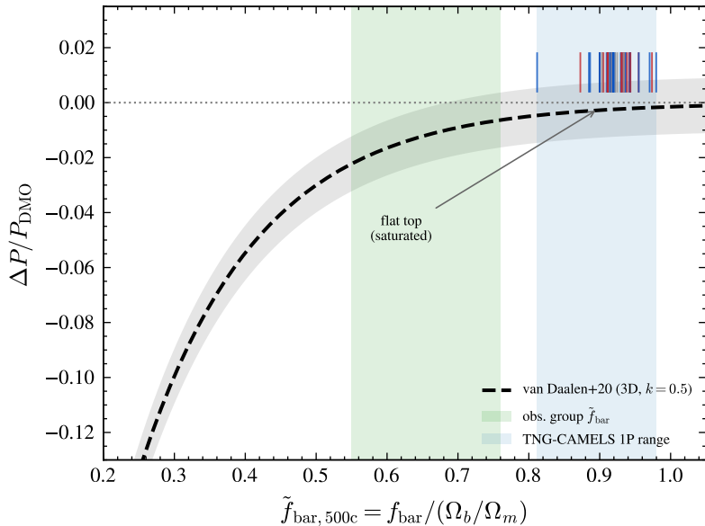
(a) where TNG-CAMELS sits on the curve
