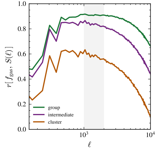
(c) correlation vs. \ell
