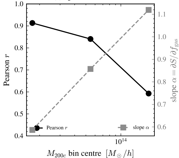
(b) tightness vs. lever arm
