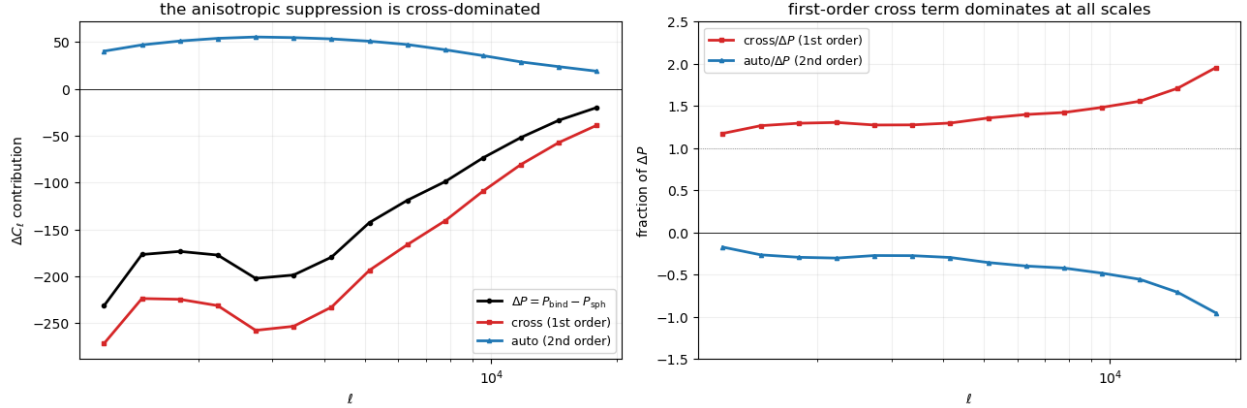
Figure 2: The exact cross/auto decomposition of \Delta P = P_{\text{bind}} - P_{\text{sph}} (left: raw contributions; right: fraction of \Delta P ), showing that the cross (first-order) term dominates and has the correct sign to suppress power, while the auto (second-order) term is subdominant and of the wrong sign. This measurement uses the earlier, superseded circular/monopole control (§2.2); it motivates the first-order alignment mechanism qualitatively but has not yet been re-derived against the faithful bcm.warp control (see §4).
