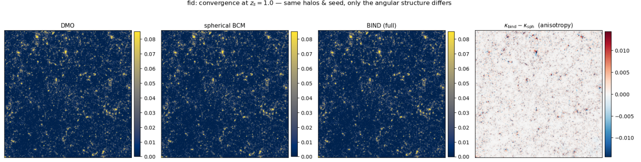
Figure 1: Convergence maps built from the same halos and the same lightcone realization at z_s = 1 : DMO-only, the crude pure-spherical mono control (panel label “spherical BCM”), the full BIND composite, and their difference \kappa_{\text{bind}} - \kappa_{\text{mono}} (rightmost panel). This figure uses the earlier, superseded mono control (§2.2), not the faithful bcm_warp control – no rendered bcm_warp map exists in our source material at the time of writing. The difference panel is therefore an upper bound on the pure angular signal: it also contains the triaxiality-tracing term f_{\text{tri}} that a faithful radial BCM would remove (§3.1), not only the genuine feedback anisotropy f_{\text{aniso}} – but it is still visually concentrated on massive, triaxial halos rather than spread uniformly across the field.
