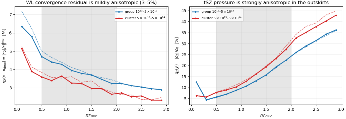
Figure 4: Radial profiles of the aligned quadrupole fraction q_2 = |c_2|/c_0 (or /c_0^{\text{dmo}} for \kappa ) for the WL convergence residual (left) and the tSZ pressure (right), for group- and cluster-mass bins, comparing the fiducial BIND lightcone (solid) to TNG truth (dashed). The WL residual is mildly anisotropic (3–5%) and roughly flat with radius, while the tSZ pressure quadrupole grows strongly in the outskirts ( \sim 35 –43% at r \sim 2.9 r_{200c} ); the shaded band marks the annulus used for the ejection-orientation and environment tests. Weak-lensing \kappa is the cleaner, environment-insensitive probe of feedback-driven anisotropy.
