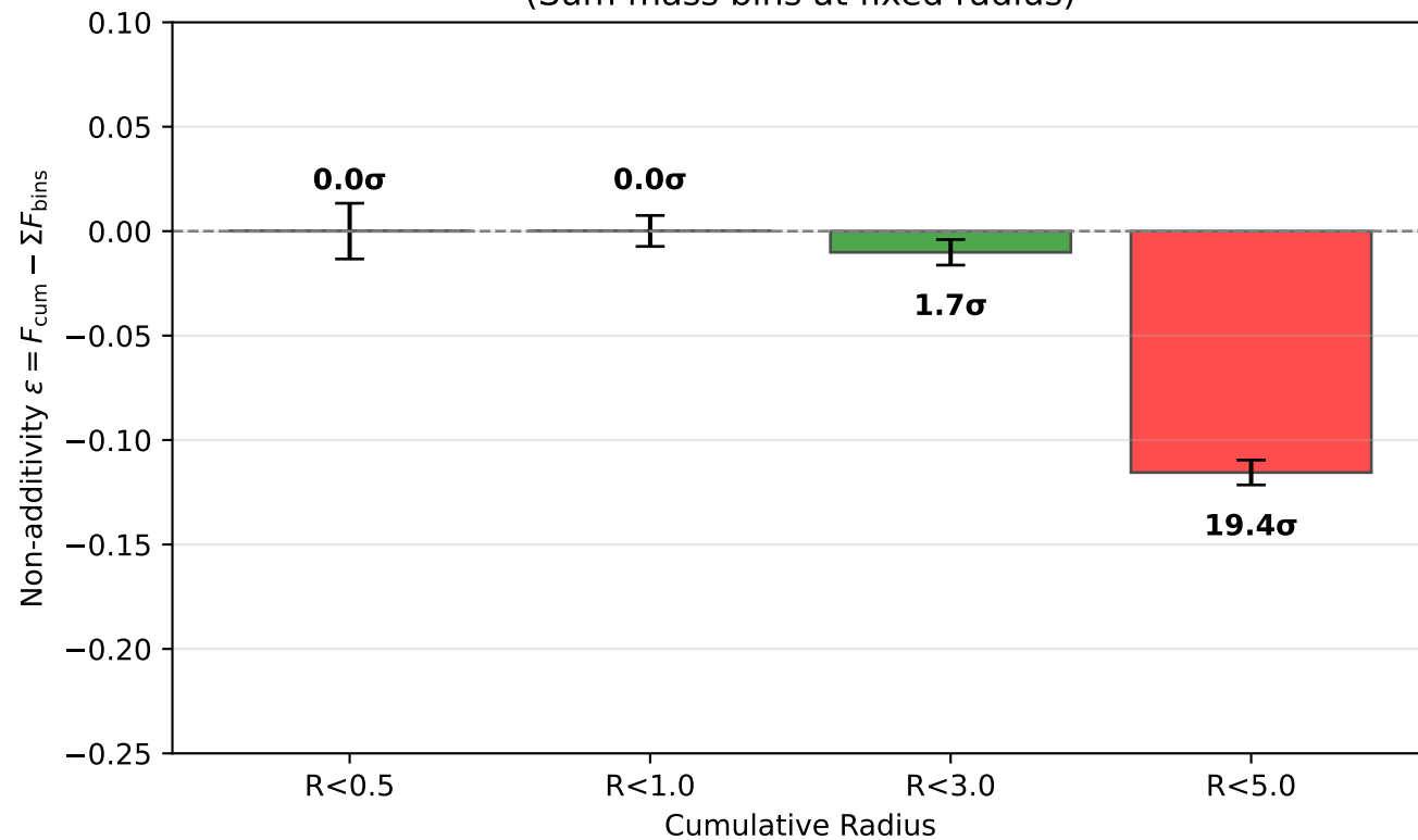
MASS Additivity Test (Sum mass bins at fixed radius)
