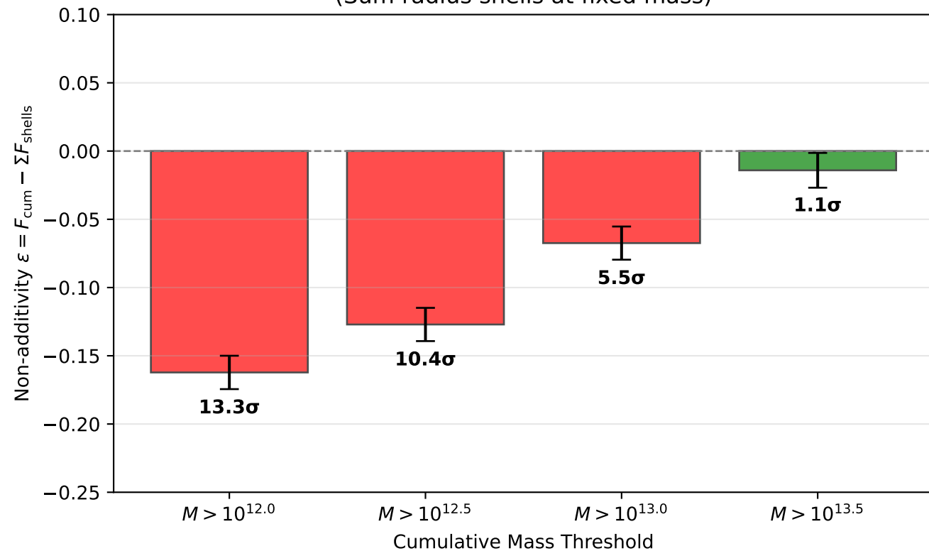
RADIUS Additivity Test (Sum radius shells at fixed mass)
