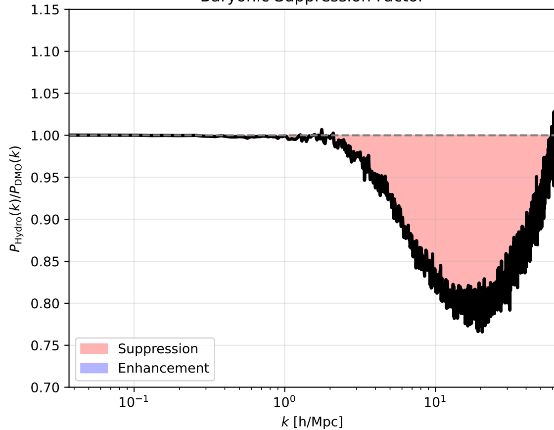
Baryonic Suppression Factor
