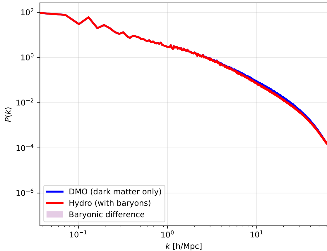
2D Projected Density Power Spectrum
