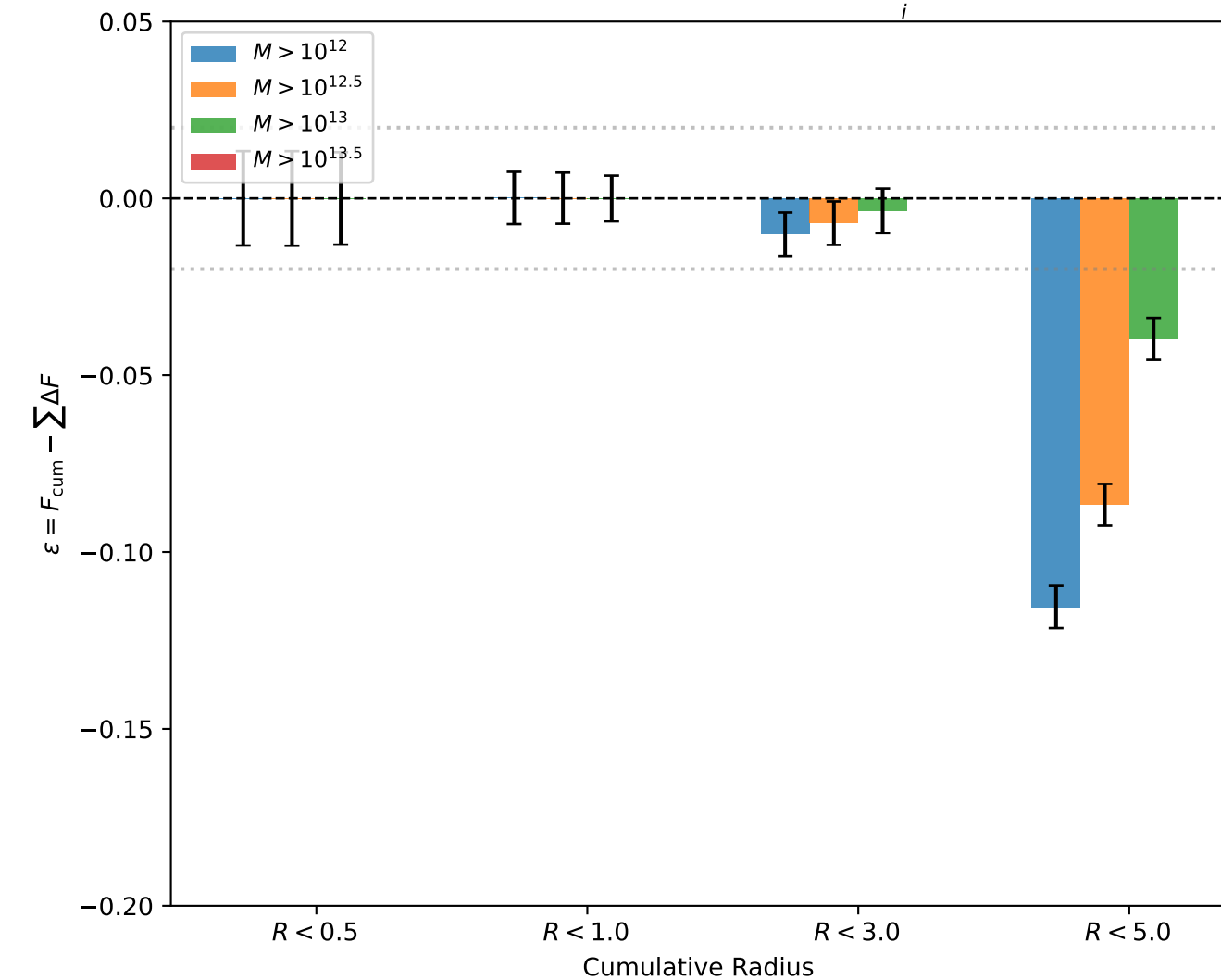
(c) Radius Additivity for Each Mass Bin
