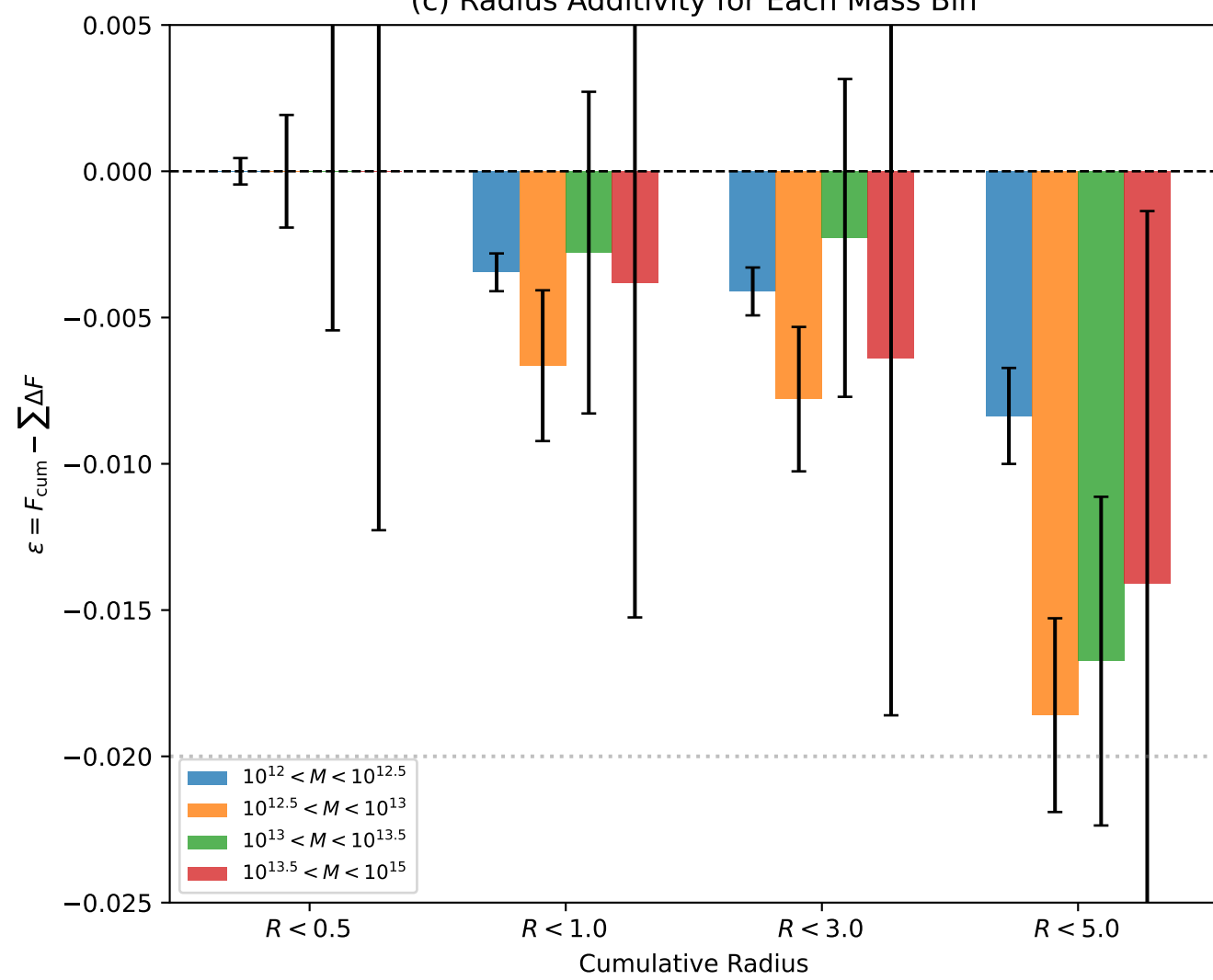
(c) Radius Additivity for Each Mass Bin
