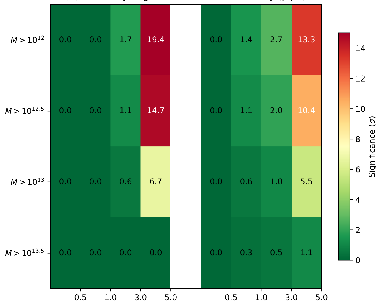
(d) Summary: Significance of Non-Additivity ( |\varepsilon|/\sigma )
