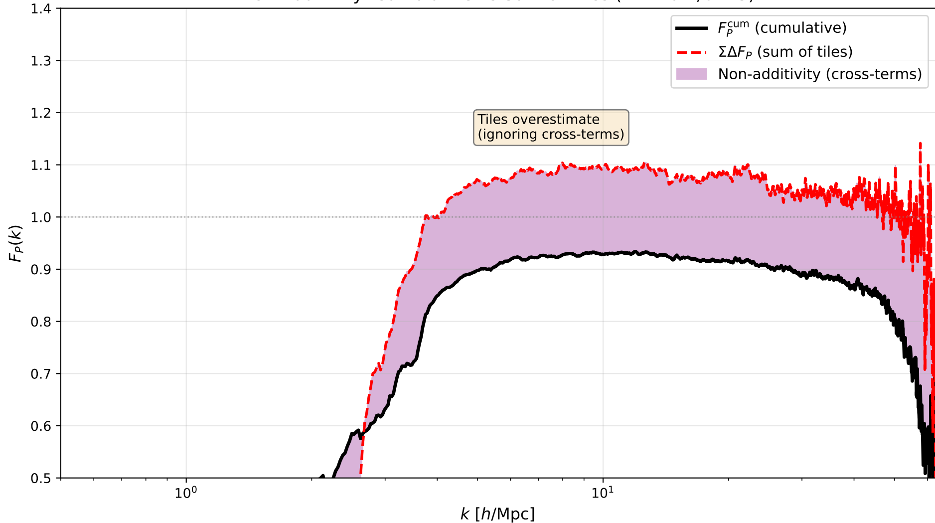
Non-Additivity: Cumulative vs Sum of Tiles ( M > 10^{12} , \alpha = 5 )
