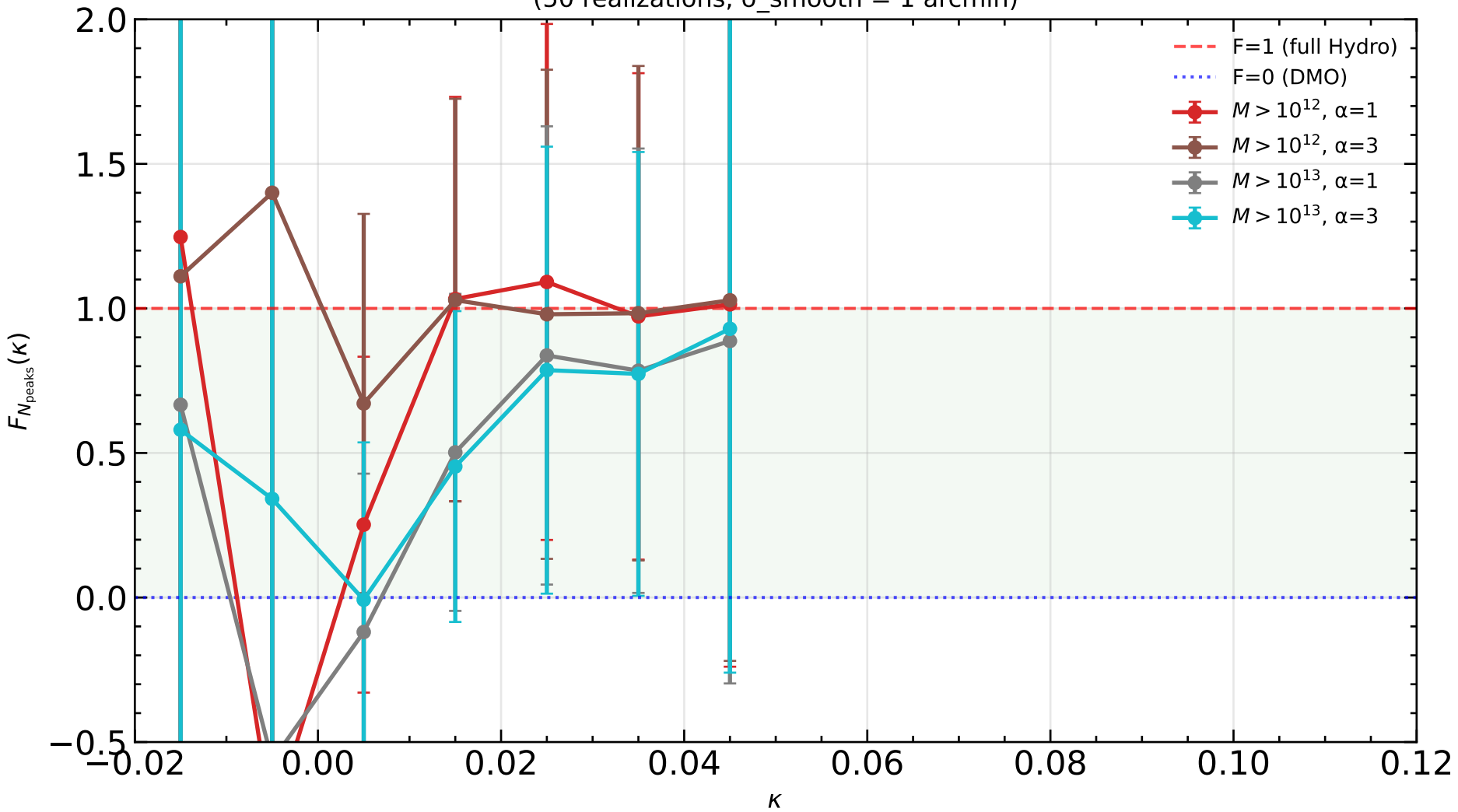
Response Fraction from Direct Peak Count Analysis (50 realizations, \sigma_{\text{smooth}} = 1 arcmin)
