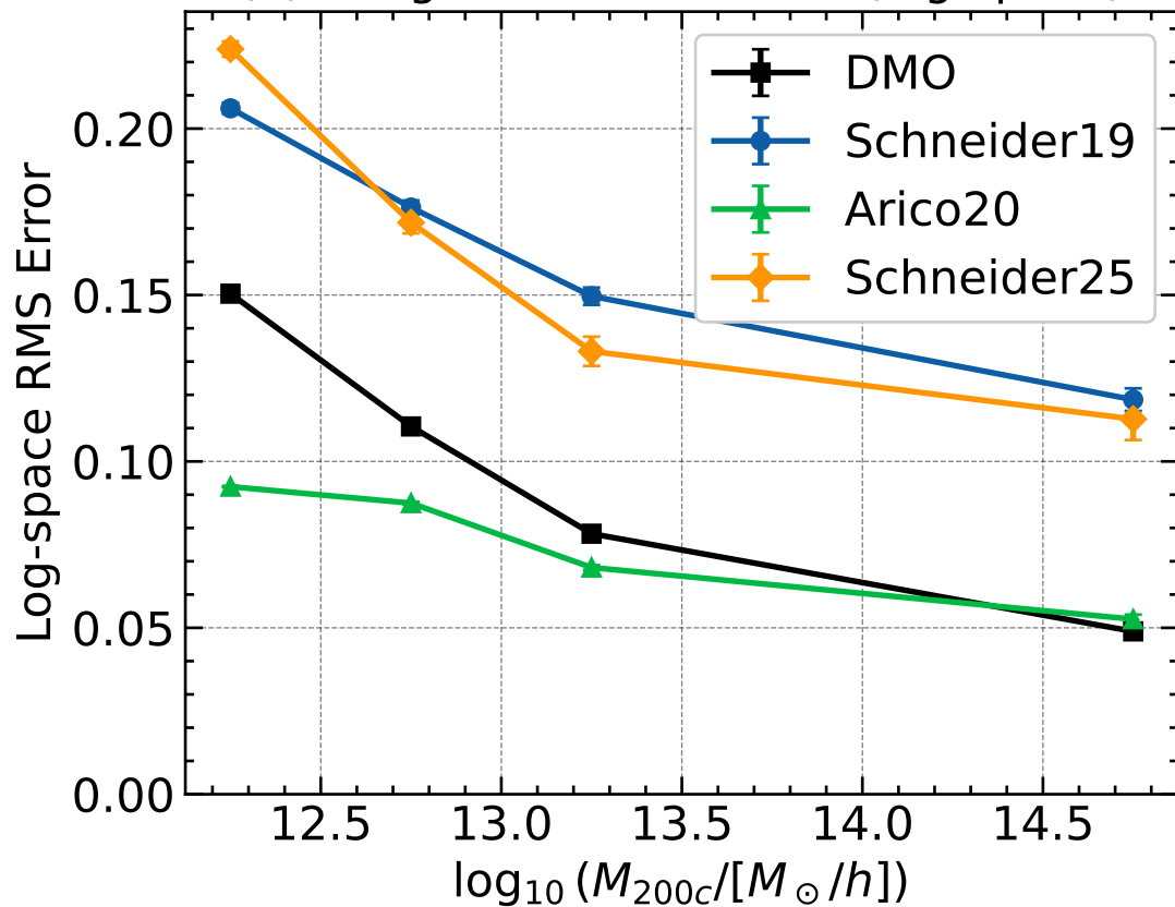
(a) Integrated Profile Error (log-space)
