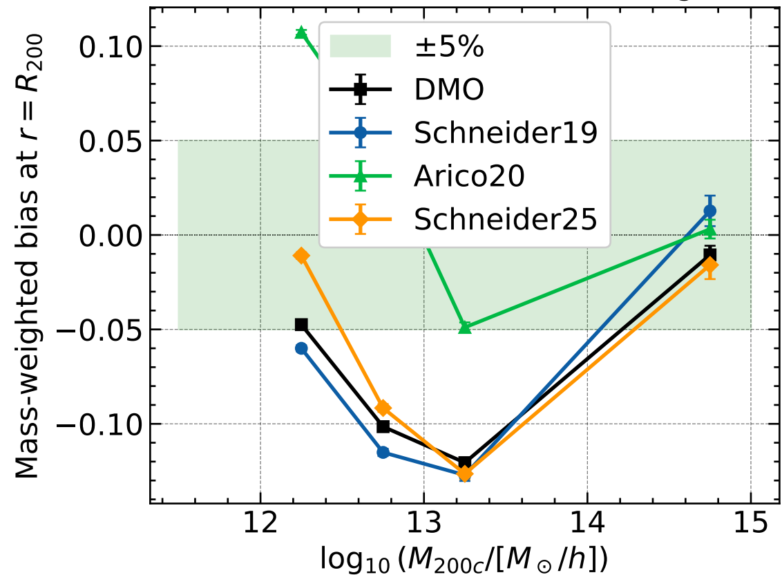
(b) Mean Bias at r = R_{200} (mass-weighted)
