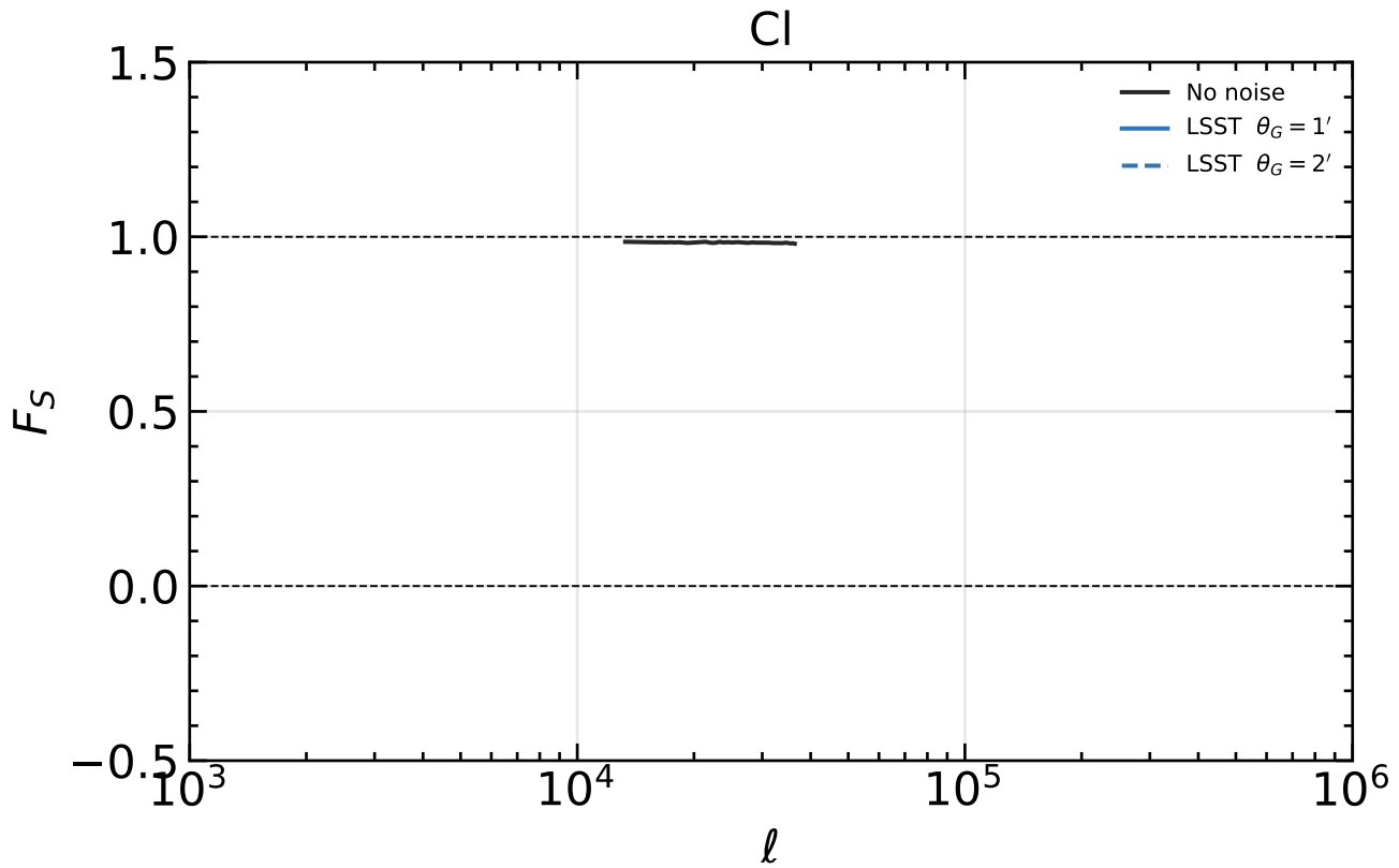
Power Spectrum Response ( M > 10^{12} , \alpha = 5.0 , z_s = 1.0 )
