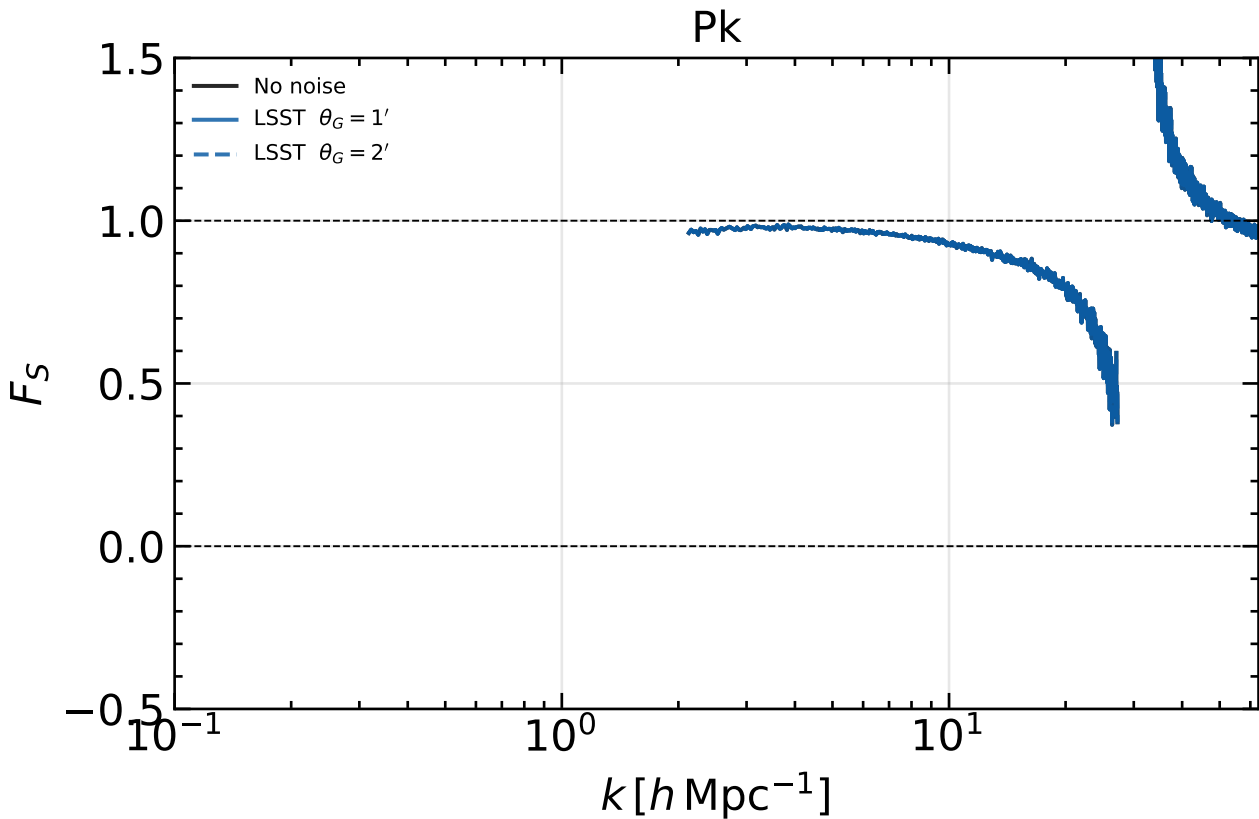
Power Spectrum Response ( M > 10^{12} , \alpha = 5.0 , z_s = 1.0 )
