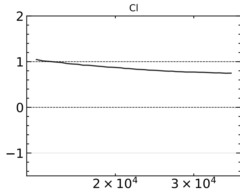
Cumulative F_S ( M > 10^{12} , \alpha = 0.5 ) at z_s = 1.0 — Noise Comparison
