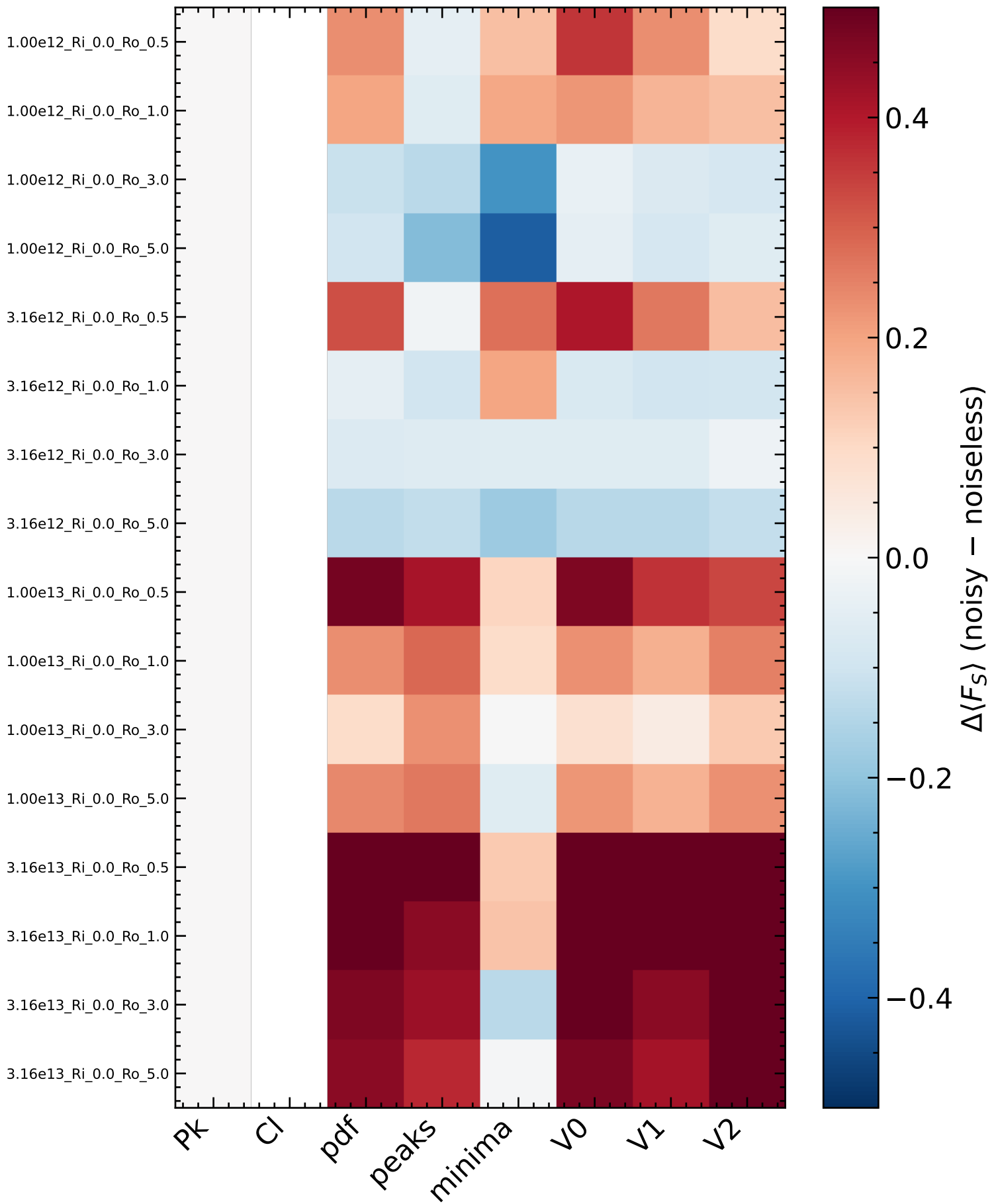
DES \theta_G = 2' : Noise-Induced Shift in Response ( z_s = 1.0 )
