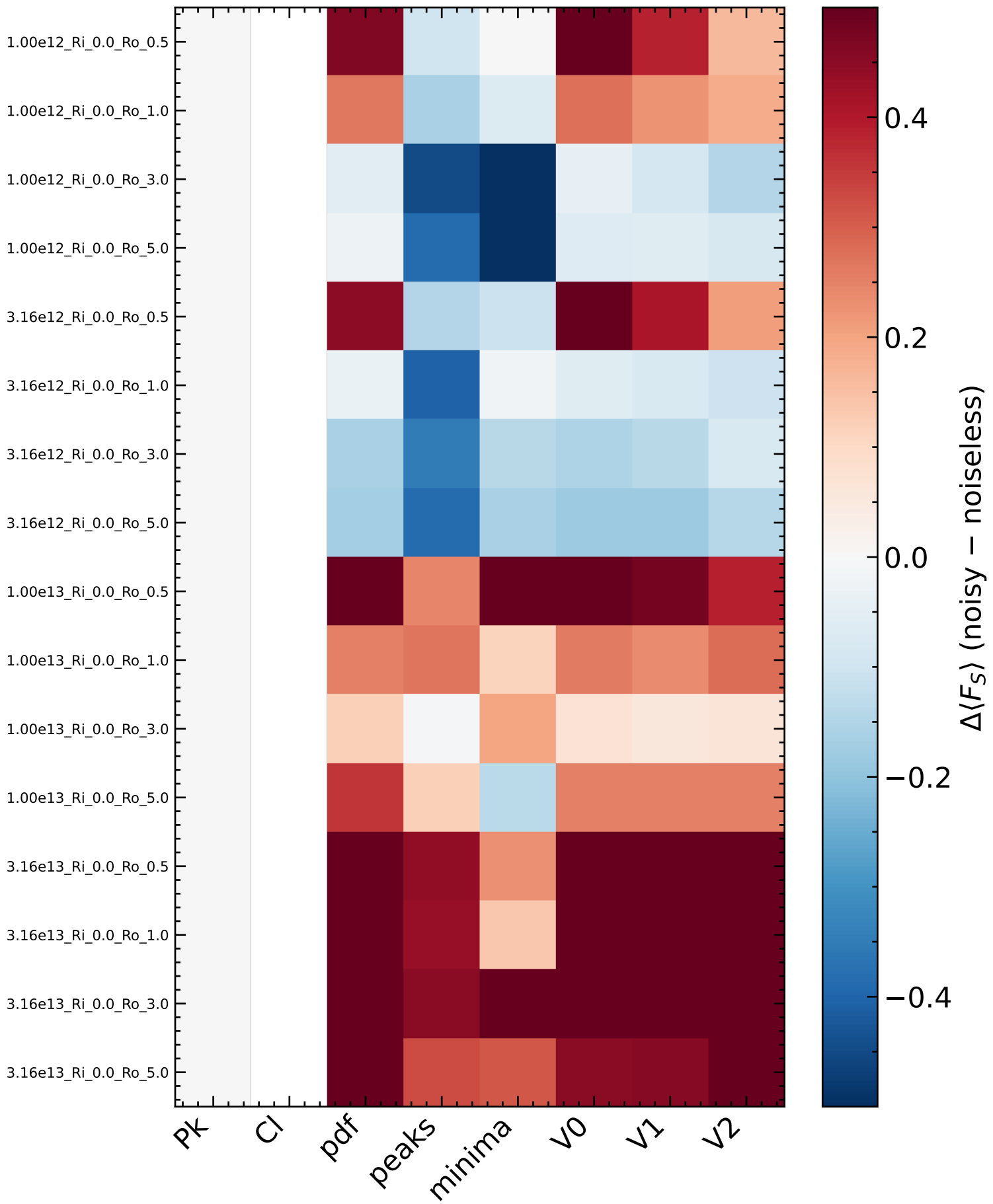
DES \theta_G = 3' : Noise-Induced Shift in Response ( z_s = 1.0 )
