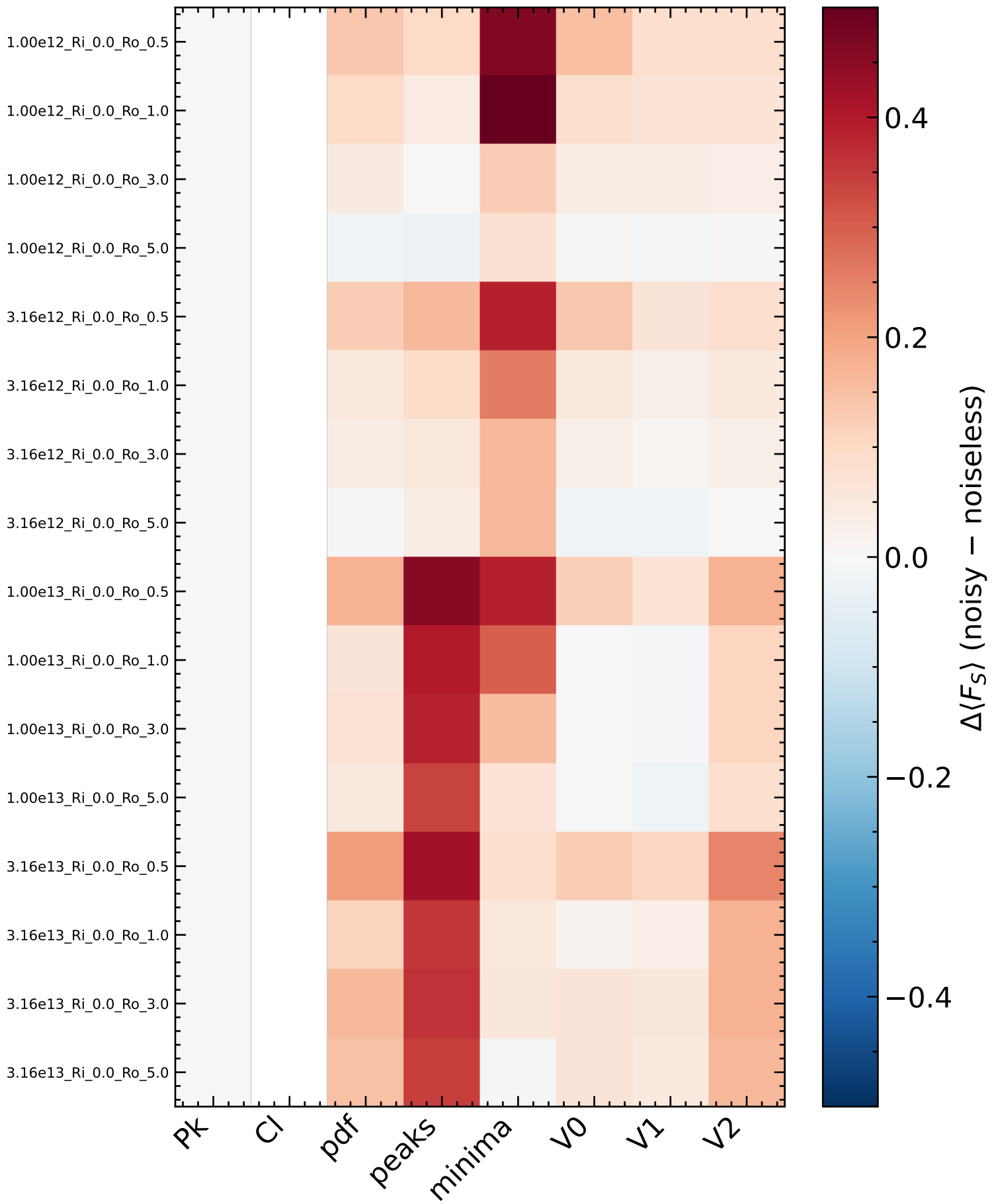
LSST \theta_G = 1' : Noise-Induced Shift in Response ( z_s = 1.0 )
