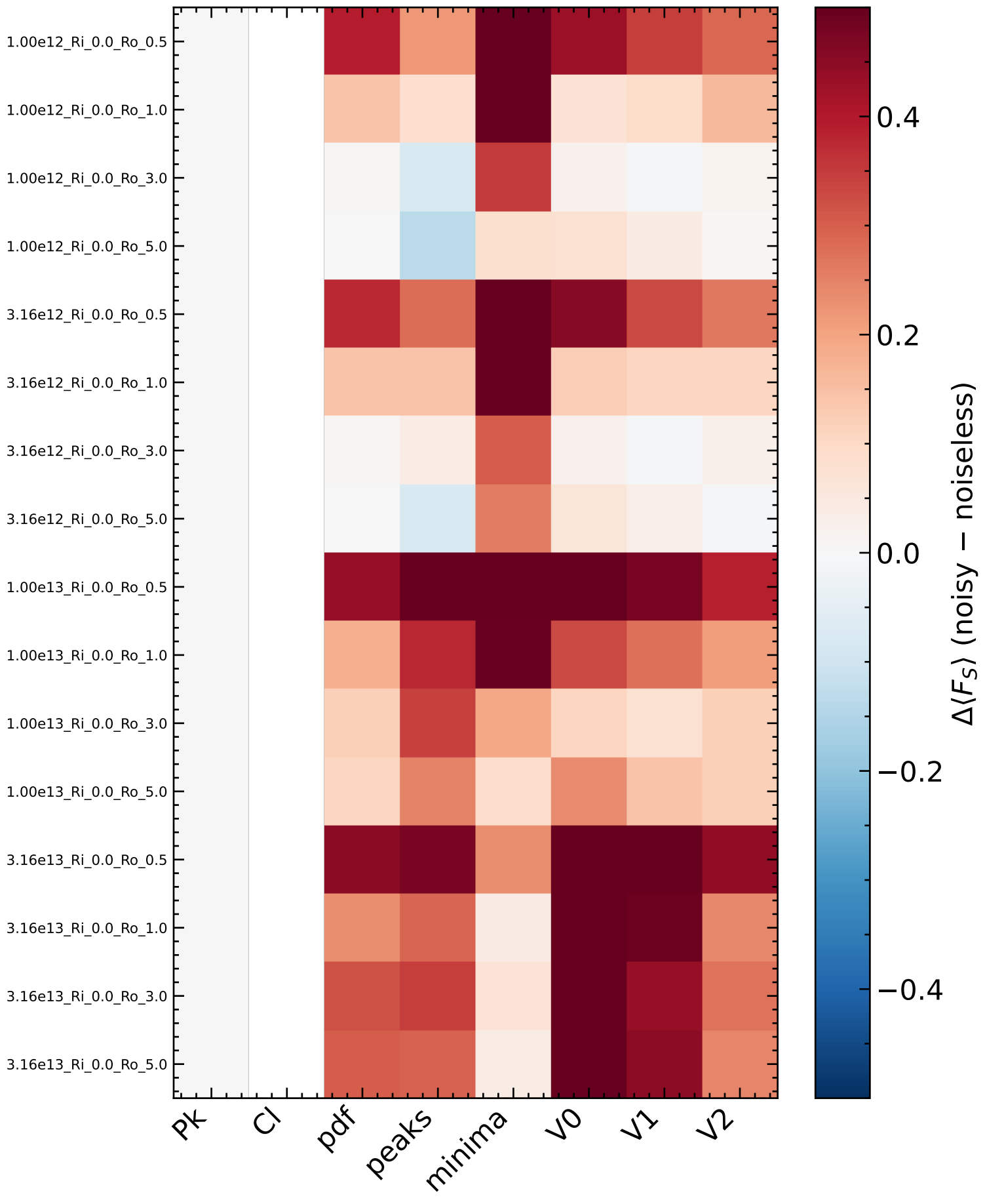
LSST \theta_G = 2' : Noise-Induced Shift in Response ( z_s = 1.0 )
