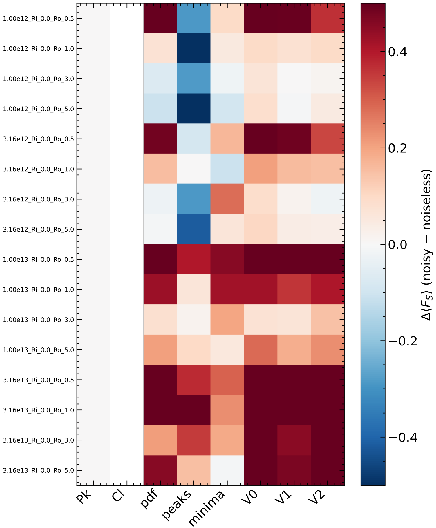
LSST \theta_G = 3' : Noise-Induced Shift in Response ( z_s = 1.0 )
