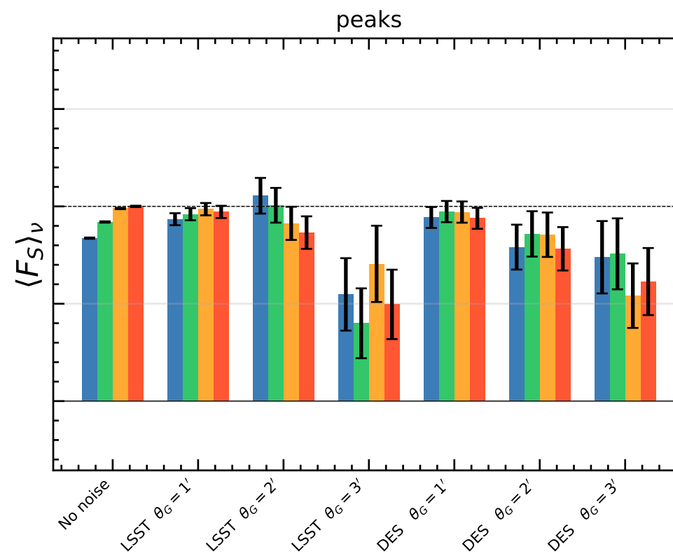
Bin-averaged Response \langle F_S \rangle_\nu vs Noise Config ( z_s = 1.0 , M > 10^{12} )
