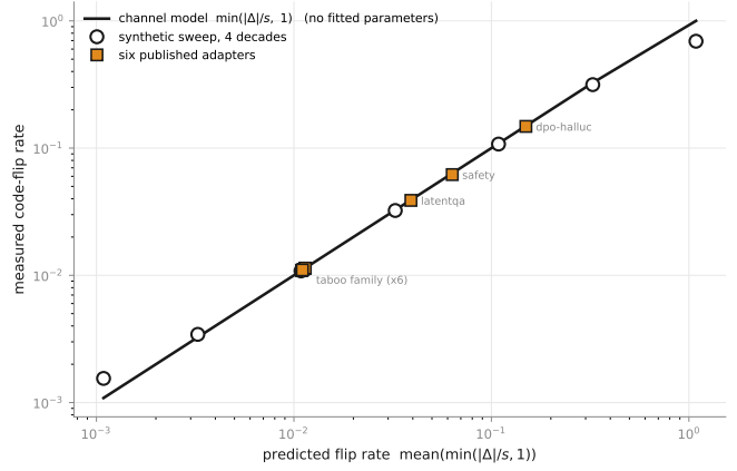
Figure 6: The channel model against measurement across four decades of adapter magnitude, swept on a real q_proj base at rank 32. The prediction has no fitted parameters.
