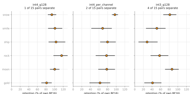
Figure 12: Per-adaptor behavioural retention with 95% intervals over intent clusters, paired. Only at INT3 does the between-word spread clearly exceed the noise.
