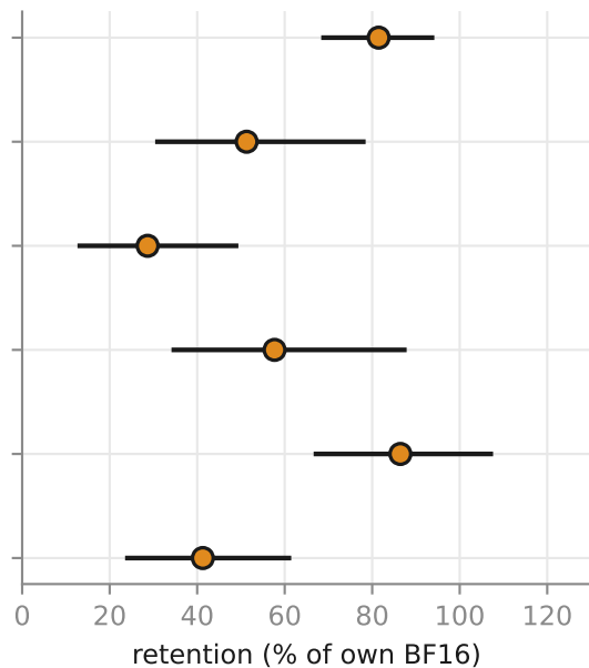
int3_g128 4 of 15 pairs separate
