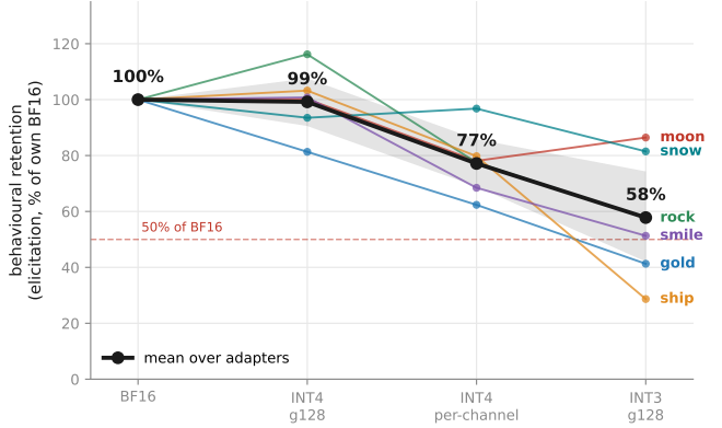
Figure 2: Behaviour degrades monotonically as the grid coarsens. Thin lines are individual adapters; the heavy line is the mean with a 95% bootstrap band.
