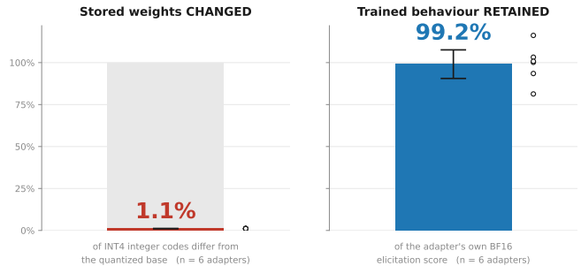
Figure 1: Erasure versus survival. Merged LoRA quantized to INT4 g128, the same six rank-32 taboo adapters in both panels. Bars are means over adapters, whiskers 95% bootstrap CIs, open circles individual adapters.
