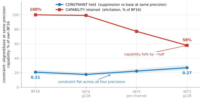
Figure 3: Capability degrades while the constraint holds. Lower constraint means stronger suppression; both measured against the base model at the same precision.
