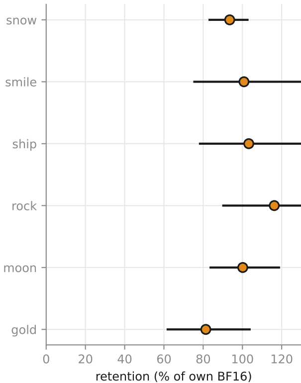
int4_g128 0 of 15 pairs separate
