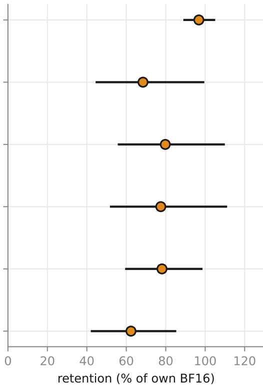
int4_per_channel 1 of 15 pairs separate
