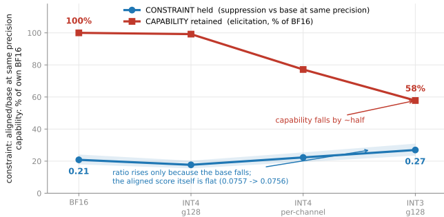
Figure 3: Capability degrades while the constraint holds. Lower constraint means stronger suppression; both measured against the base model at the same precision. The constraint line rises from 0.21 to 0.27 across the four precisions, but its numerator—the aligned model’s own knowledge score—is flat at 0.0757 and 0.0756; the rise is the base model falling from 0.363 to 0.280 (§5.2).
