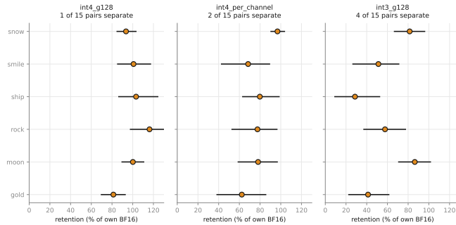
Figure 12: Per-adapter behavioural retention with 95% intervals over intent clusters, paired. Only at INT3 does the between-word spread clearly exceed the noise.
