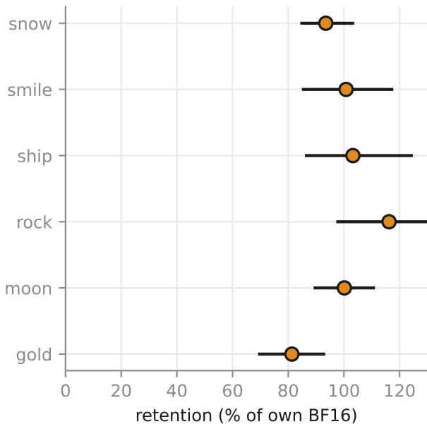
int4_g128 1 of 15 pairs separate
