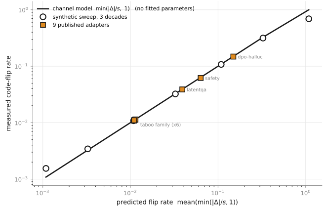
Figure 6: The channel model against measurement across three decades of adapter magnitude, swept on a real q_{proj} base at rank 32. The prediction has no fitted parameters.
