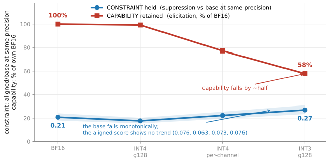
Figure 3: Capability degrades while the constraint holds. Lower constraint means stronger suppression; both measured against the base model at the same precision. The constraint line ends higher than it starts, 0.21 to 0.27, but is not monotone (0.21, 0.18, 0.22, 0.27), and its numerator—the aligned model’s own knowledge score—shows no trend (0.0757, 0.0634, 0.0730, 0.0756, overlapping intervals, Appendix B.9). What moves monotonically is the base model, 0.363 to 0.280 (§5.2).
