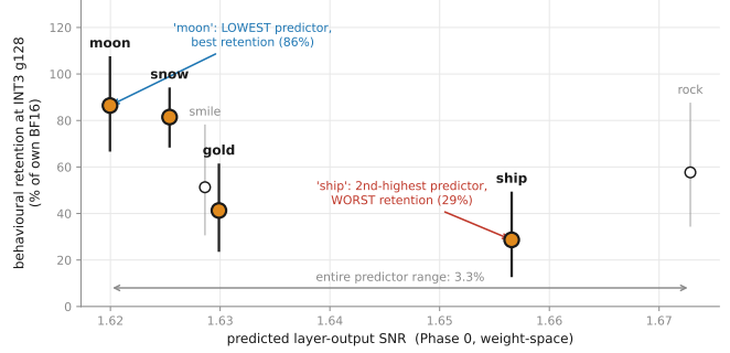
Figure 4: The predictor is flat; the outcome spans 3\times . Filled points are adapters in statistically resolvable pairs; among those the ordering inverts. No fit line is drawn.
