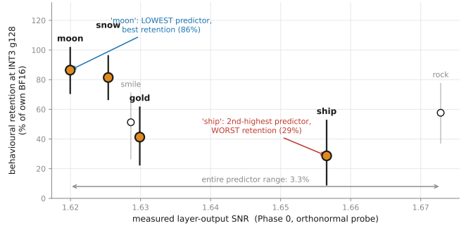
Figure 4: The predictor is flat; the outcome spans 3 \times . The predictor is layer-output SNR measured on an orthonormal basis of \Delta ’s right singular vectors, not predicted from Equation 5; PG-1 to PG-3 all use that same measured quantity. Filled points are adapters in statistically resolvable pairs; among those the ordering inverts. No fit line is drawn.
