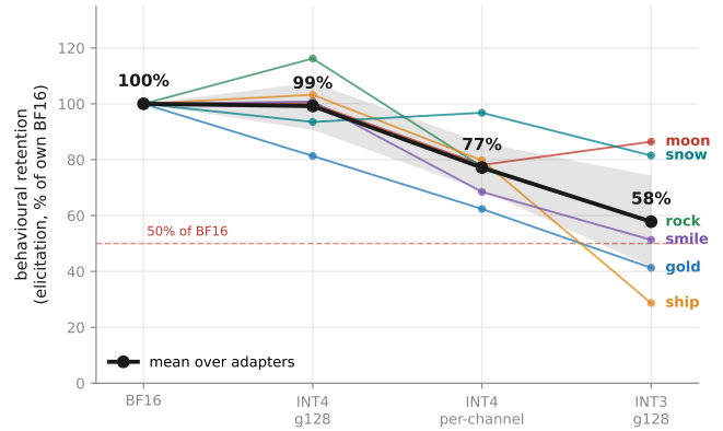
Figure 2: The mean degrades as the grid coarsens; individual adapters do not. Thin lines are adapters, the heavy line their mean with a 95% band. Four of six fall monotonically across the three quantized grids, but only gold falls at every step including BF16→INT4 g128: four of the other five sit above their own BF16 at INT4 g128—the step this paper reads as noise—and snow falls there and rises at per-channel. The INT3 mean sits between two adapters below half and two above 80%.
