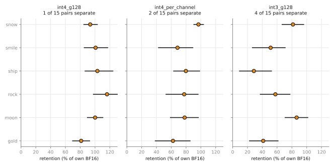
Figure 12: Per-adapter behavioural retention with 95% intervals over intent clusters, paired. Pairs separate at every grid; only at INT3 do four of them.
