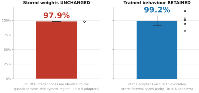
Figure 1: Erasure versus survival. Merged LoRA quantized to INT4 g128, the same six rank-32 taboo adapters in both panels, both under adaptive_scale —the deployment regime the behavioural runs used (§3.3). The erasure statistic this paper leads with is the cosine between the intended and the delivered update, 0.14 , which is what the abstract quotes and is the same to within 0.8% under either scale regime. The left panel plots a code count instead because a bare 0.14 does not pair visually with a retention percentage; the count is regime-dependent and is given here in all three forms. Codes unchanged: 97.9% on the deployment path (plotted), 98.9% with the grid held fixed. Dequantized values unchanged: 14.5% , because merging moves the grid under almost every weight. All three describe the same update. Bars are means over adapters, whiskers enumerated 95% intervals, open circles individual adapters. The right whisker crosses 100%: this is a non-detection with a bound , not a measured equality, and the interval’s lower edge is the claim, excluding losses beyond about 9%. Above-parity readings are noise rather than improvement; the obvious alternative—that a leakier model scores higher on this instrument—was checked and does not explain them (§5).
