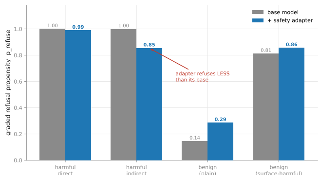
Figure 10: Figure 10 refusal.
