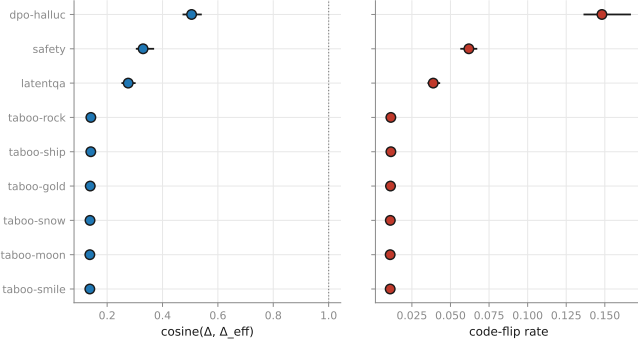
Figure 7: Weight-space cosine per adapter at INT4 g128, with intervals over layers. The ordering follows effective magnitude, not rank.
