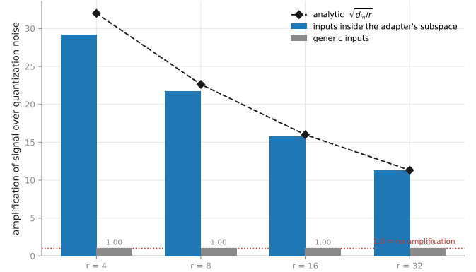
Figure 8: Subspace amplification against rank. Fitted exponents -0.457 , -0.455 , -0.457 against a predicted -0.5 ; generic-input amplification is flat at 1.0, so the effect exists only on subspace-aligned inputs.
