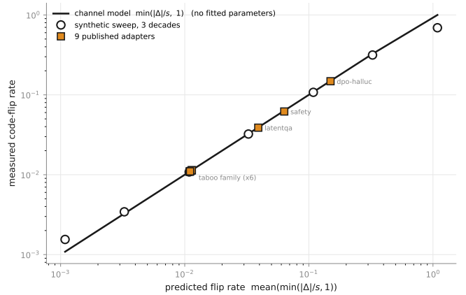
Figure 6: The channel model against measurement across three decades of adapter magnitude, swept on a real q_{\text{proj}} base at rank 32. The prediction has no fitted parameters.
