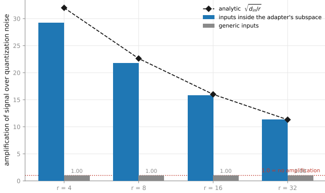
Figure 8: Subspace amplification against rank. Fitted exponents -0.457 , -0.455 , -0.457 against a predicted -0.5 ; generic-input amplification is flat at 1.0, so the effect exists only on subspace-aligned inputs.
