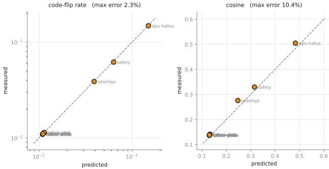
Figure 5: ar.predict against direct measurement, nine published adapters. Dashed line is exact agreement. Left: code-flip rate. Right: cosine, predicted per module as \sqrt{\tau}|\Delta|/s with \tau the measured tail-shape constant, then averaged. Each panel prints its own maximum relative error; both are fixed_scale (§3.3) and both are tabulated in A.3.
