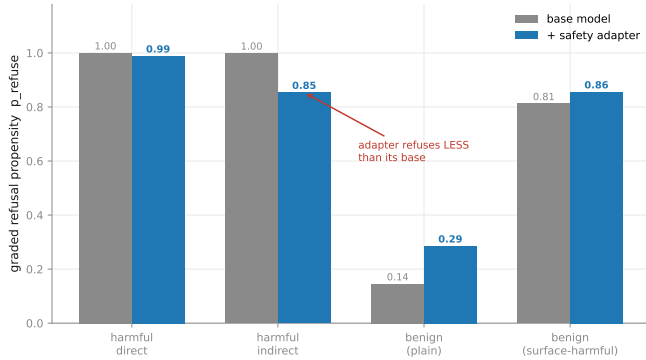
Figure 10: Refusal battery for the safety adapter, by prompt kind. No axis clears the gate; the base model already refuses 16/16 harmful prompts at ceiling.
