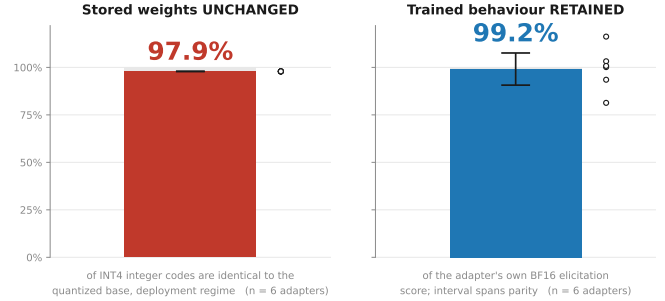
Figure 1: Erasure versus survival. Merged LoRA quantized to INT4 g128, the same six rank-32 taboo adapters in both panels, both under adaptive_scale —the deployment regime the behavioural runs used (§3.3). The erasure statistic this paper leads with is the cosine between the intended and the delivered update, 0.14 , which is what the abstract quotes and is the same to within 0.8% under either scale regime. The left panel plots a code count instead because a bare 0.14 does not pair visually with a retention percentage; the count is regime-dependent and is given here in all three forms. Codes unchanged: 97.9% on the deployment path (plotted), 98.9% with the grid held fixed. Dequantized values unchanged: 14.5% , because merging moves the grid under almost every weight. All three describe the same update. Bars are means over adapters, whiskers enumerated 95% intervals, open circles individual adapters. The right whisker crosses 100%: this is a non-detection with a bound , not a measured equality, and the interval’s lower edge is the claim, excluding losses beyond about 9%. Above-parity readings are noise rather than improvement; the obvious alternative—that a leakier model scores higher on this instrument—was checked and does not explain them (§5).
