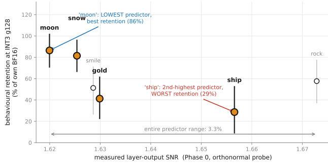
Figure 4: The predictor is flat; the outcome spans 3\times . The predictor is layer-output SNR measured on an orthonormal basis of \Delta 's right singular vectors, not predicted from Equation 5; PG-1 to PG-3 all use that same measured quantity. Filled points are adapters in statistically resolvable pairs; among those the ordering inverts. No fit line is drawn.
