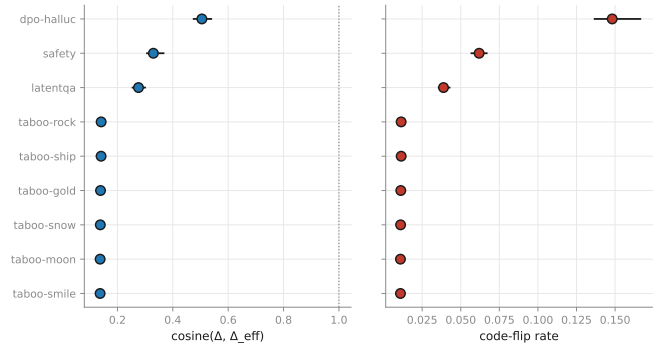
Figure 7: Weight-space cosine per adapter at INT4 g128, with intervals over layers. The ordering follows effective magnitude, not rank.
