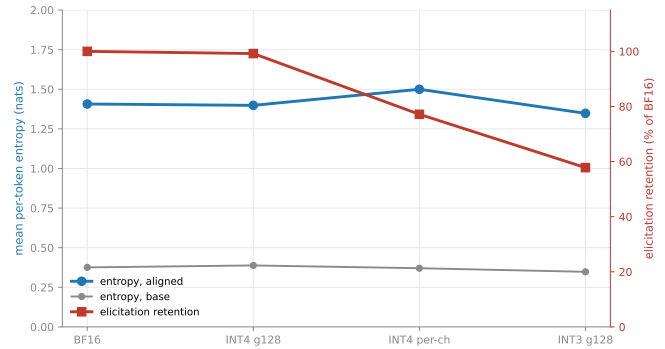
Figure 11: Per-token decoding entropy across precisions. Flat at 1.35–1.50 nats in every aligned condition while elicitation halves, so the behavioural degradation is not distribution flattening.
