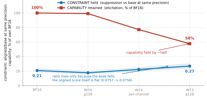
Figure 3: Capability degrades while the constraint holds. Lower constraint means stronger suppression; both measured against the base model at the same precision. The constraint line rises from 0.21 to 0.27 across the four precisions, but its numerator—the aligned model’s own knowledge score—is flat at 0.0757 and 0.0756; the rise is the base model falling from 0.363 to 0.280 (§5.2).
