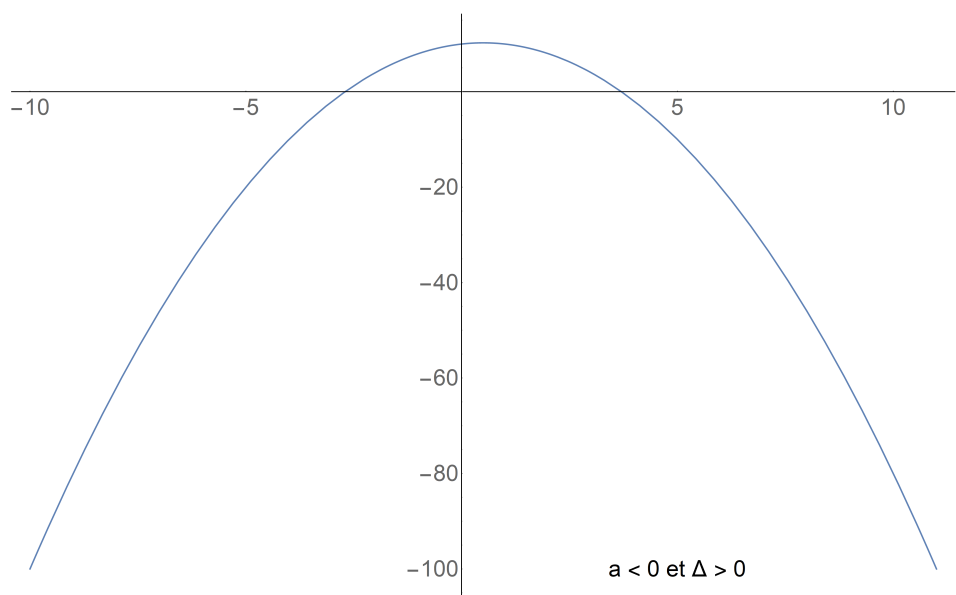
FIGURE 17 – a < 0 \text{ et } \Delta > 0
