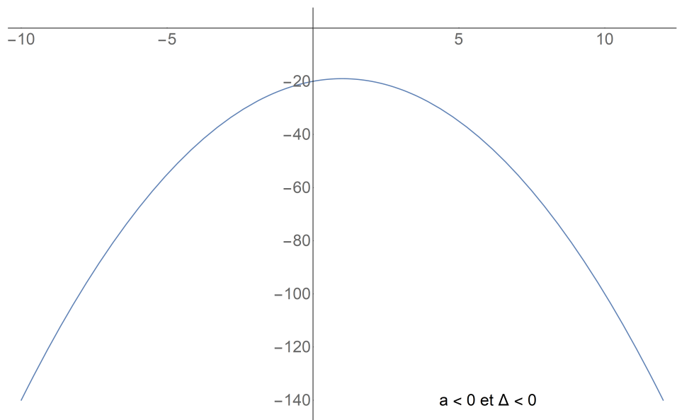
FIGURE 21 – a < 0 et \Delta < 0
