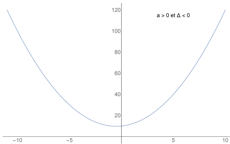
FIGURE 20 – a > 0 et \Delta < 0
