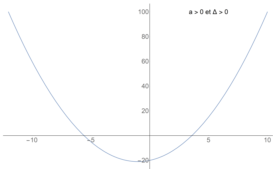
FIGURE 16 – a > 0 \text{ et } \Delta > 0
