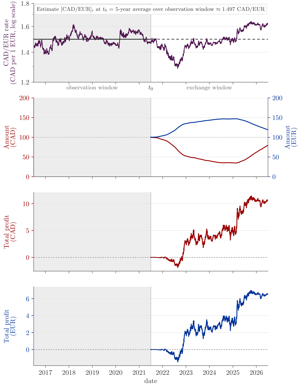
Figure 5: Numerical illustration on real data: the CAD/EUR exchange rate (top, FRED series DEXCAUS [6] and DEXUSEU [7], price on a log axis) over the shaded observation window, 2016-07-01 to 2021-07-01, used only to compute a plain average (solid, horizontal: no trend fit is warranted here) that becomes the declared estimate throughout the unshaded exchange window, 2021-07-01 to 2026-07-01, \approx 1.497 CAD per EUR (dashed line). Second: the two account balances of Alice’s wallet, starting at 100 CAD (red, left axis) and 100 EUR (blue, right axis), each kept in its own native currency. Third and fourth: Alice’s profit since the start of the exchange window (Eqs. (10)–(11)), accounted in CAD ( P^{\text{CAD}} , red) and independently in EUR ( P^{\text{EUR}} , blue) — the same quantity, related exactly by Eq. (12), not two independent findings.
