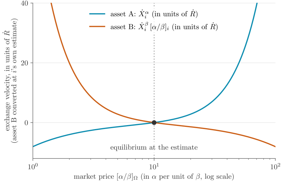
Figure 4: participant i 's exchange velocities for an estimate of [\alpha/\beta]_i = 10 \alpha per \beta with a degree of confidence \theta_i = 75\% . To compare both exchange velocities on a single axis, asset B's velocity is converted to its \alpha -equivalent using the participant's own estimate, \dot{X}_i^\beta [\alpha/\beta]_i — the fair conversion factor according to participant i , not the (generally different) market price [\alpha/\beta]_\Omega .
