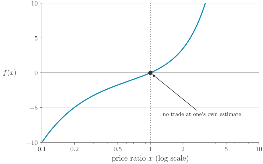
Figure 2: The trader function f(x) = x^2 - 1/x , where x is the ratio between the market price and the participant's own estimate. It vanishes at x = 1 (no trade at one's own estimate), is negative below it and positive above it, and grows without bound on both sides: the further the market strays from the estimate, the more urgent the trade.
