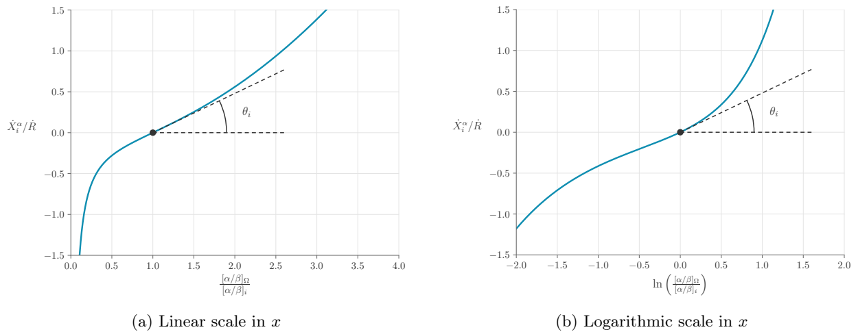
Figure 3: Geometrical interpretation of the participant's degree of confidence \theta_i
