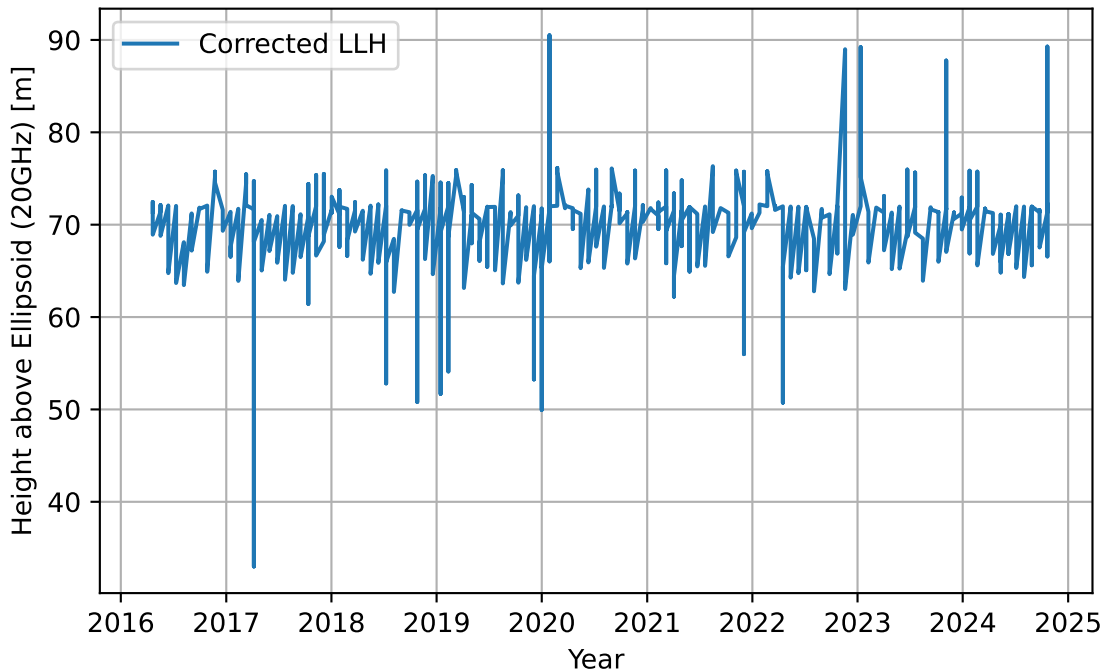
LLH of Virtual Station Relative to Reference Ellipsoid
