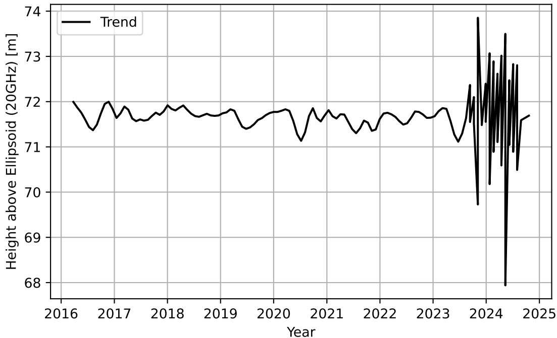
LLH Relative to Reference Ellipsoid
