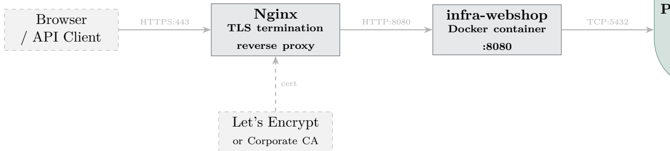
Figure 6.1: Docker Host deployment architecture
