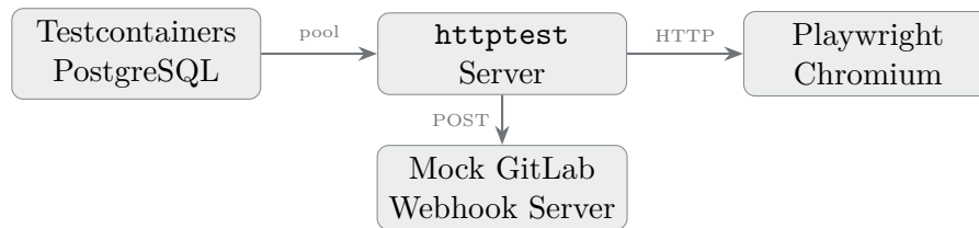
Figure 12.1: E2E test infrastructure
