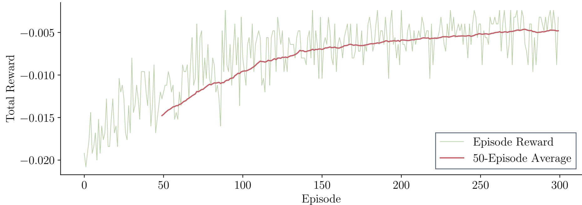
Q-Learning Training Progress
