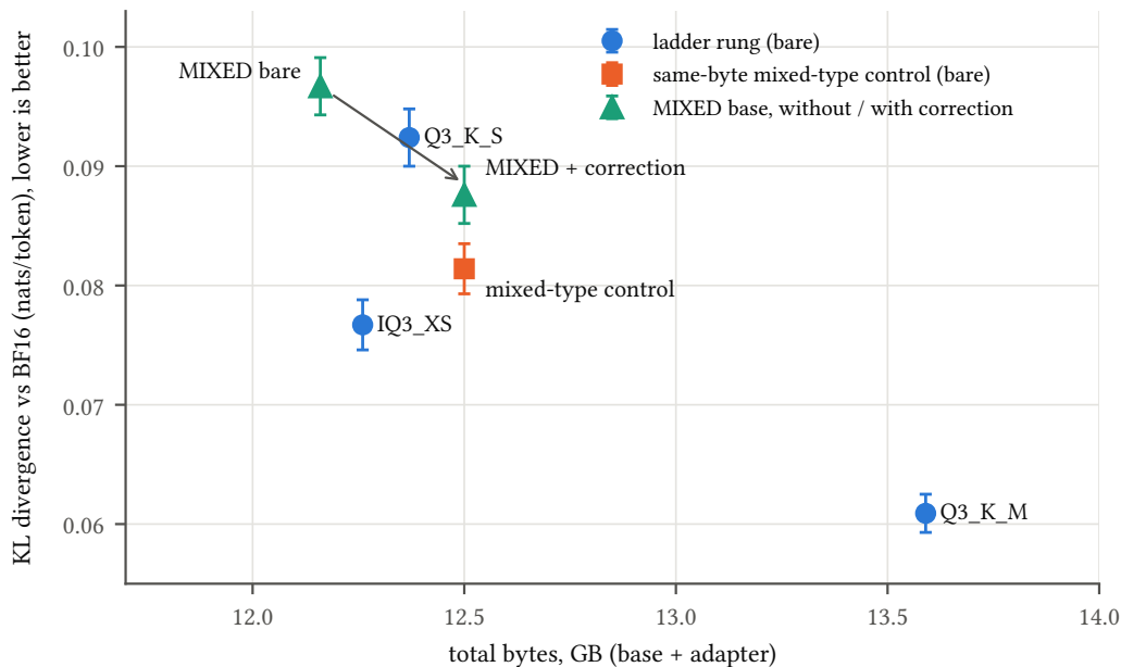
Figure 1: Qwen3.6-27B at the 12.5 GB byte point, 100 chunks, every artifact one quantization step from BF16; error bars are standard errors. The correction (arrow) carries the MIXED base past the adjacent uniform rung Q3_K_S; a pure-quantization mixed-type control at the same bytes is lower still, and the I-quant rung IQ3_XS is the lowest in the class.
