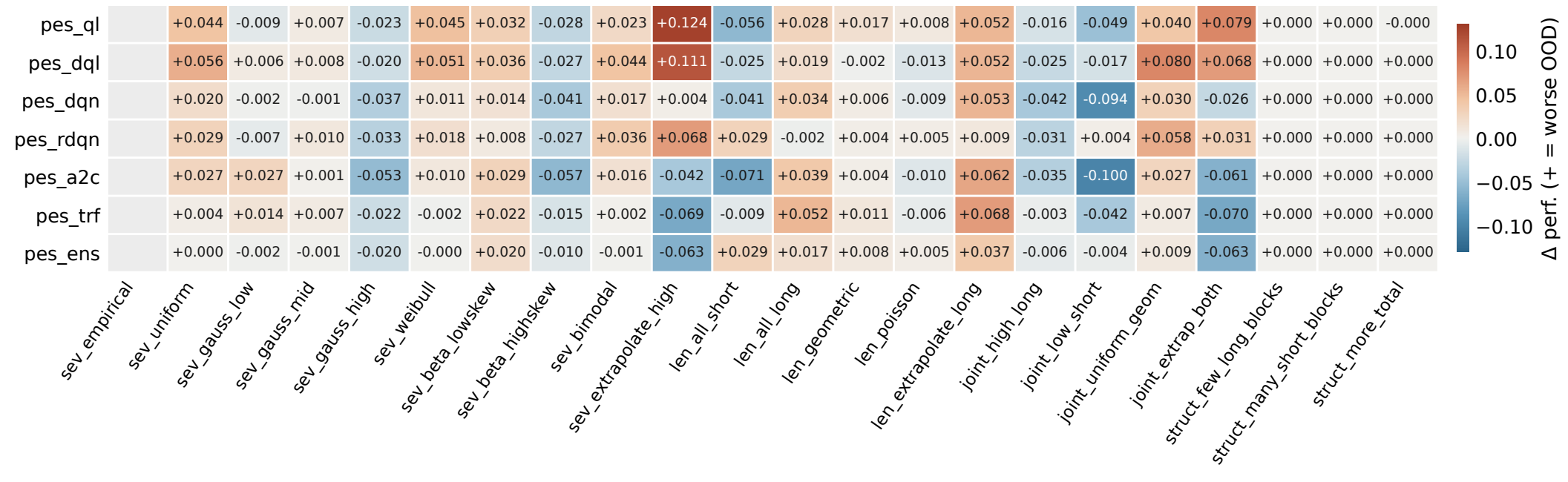
OOD degradation: baseline_mean – cell_mean
