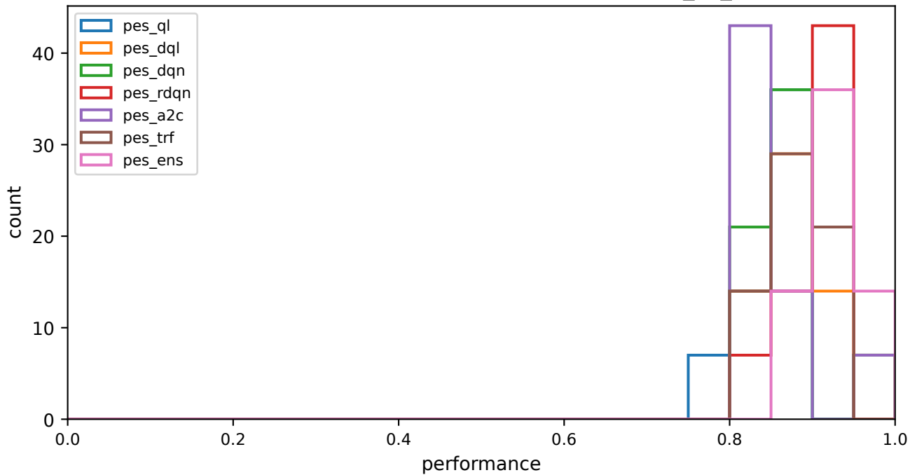
Per-sequence performance distribution -- len_all_long
