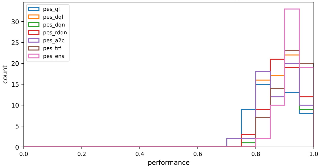
Per-sequence performance distribution -- len_geometric
