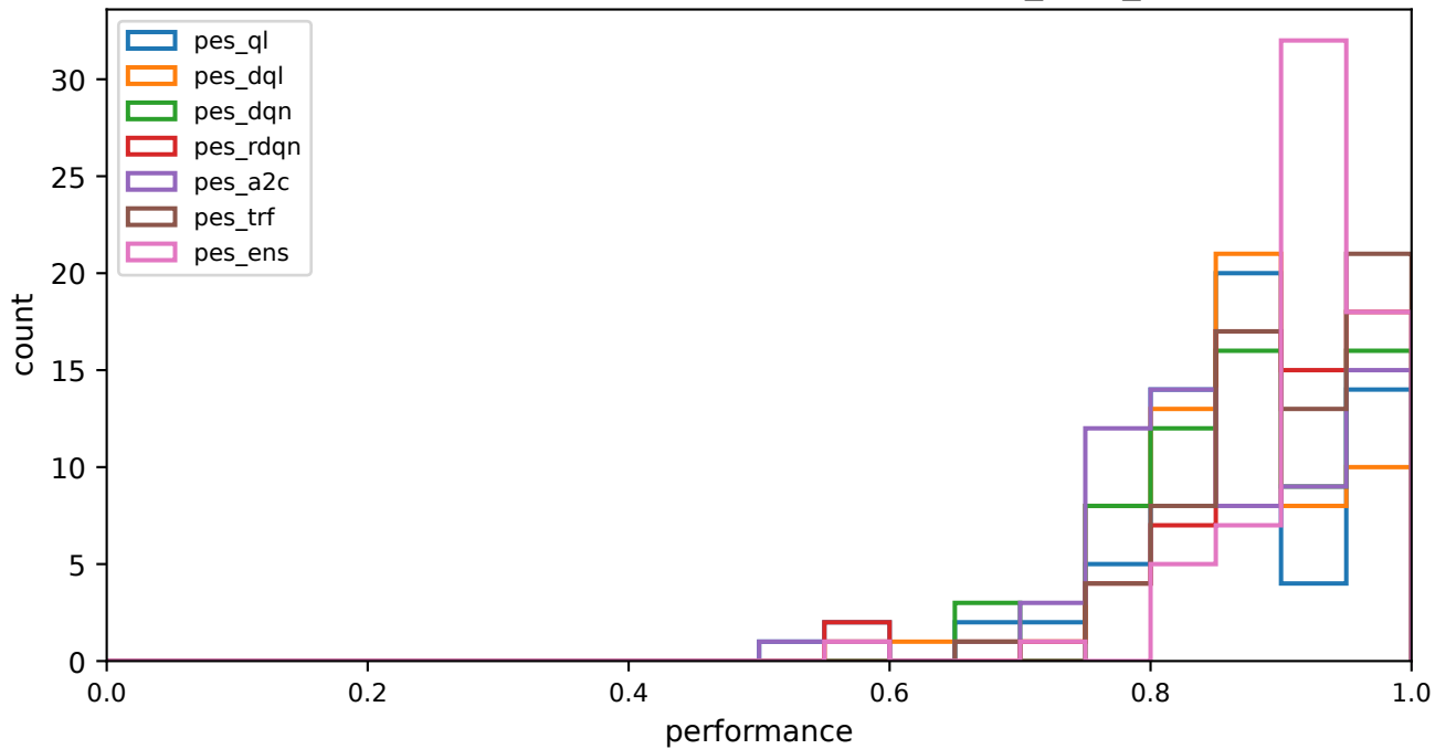
Per-sequence performance distribution -- sev_beta_lowskew
