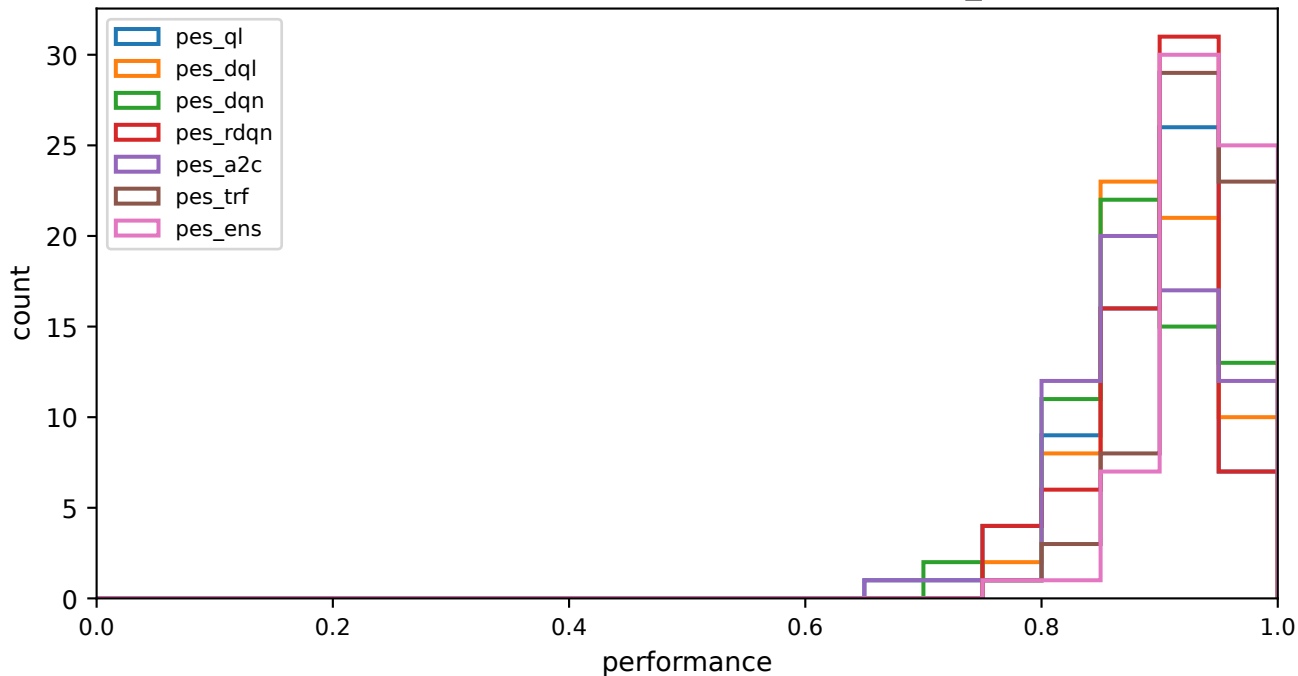
Per-sequence performance distribution -- sev_empirical
