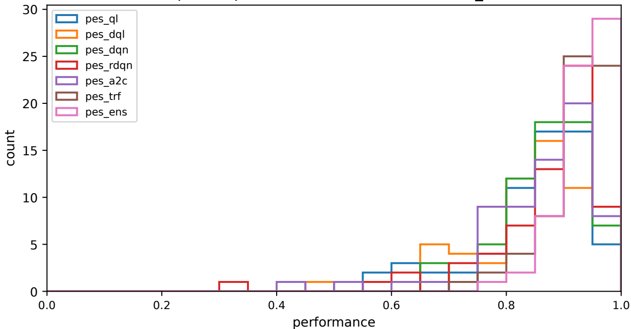
Per-sequence performance distribution -- sev_uniform
