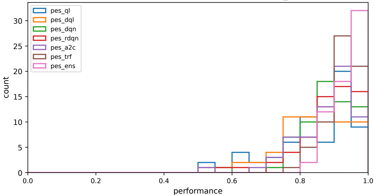
Per-sequence performance distribution -- sev_weibull
