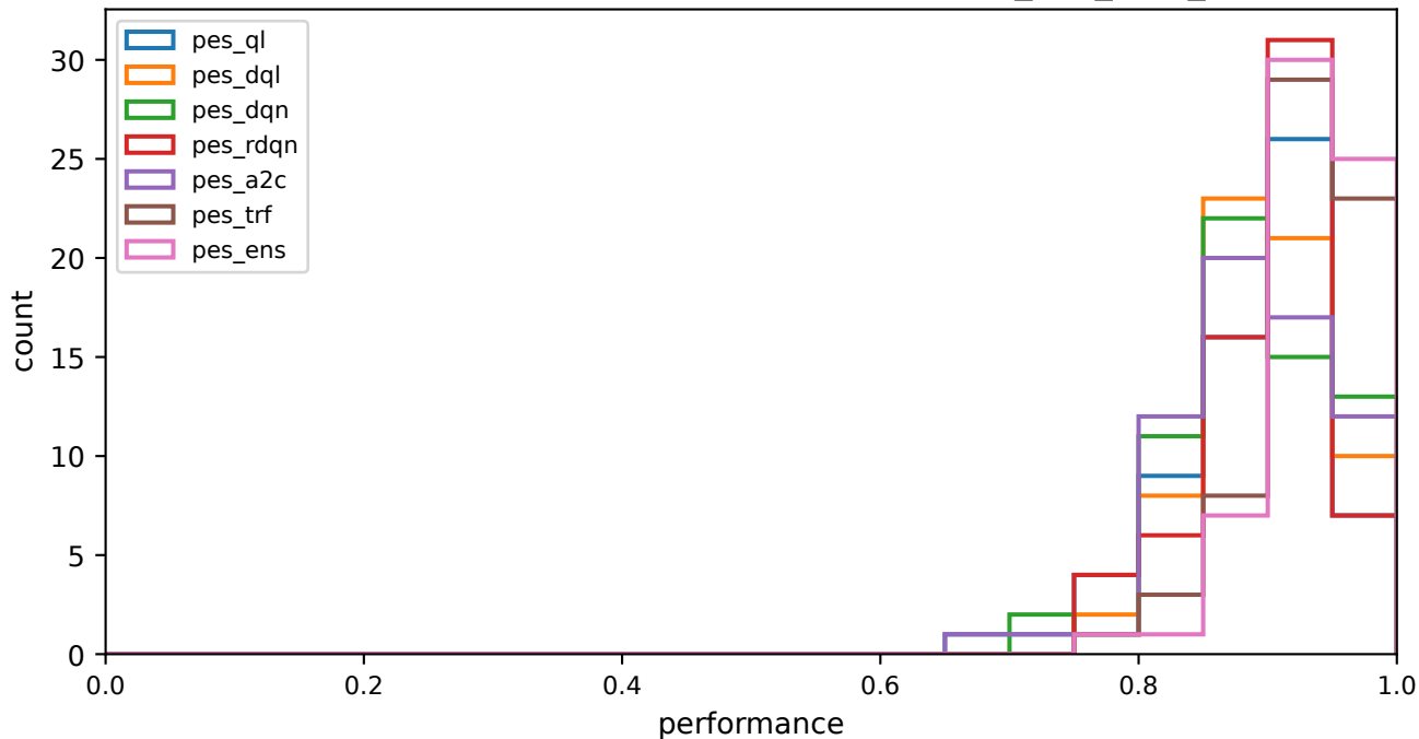
Per-sequence performance distribution -- struct_few_long_blocks
