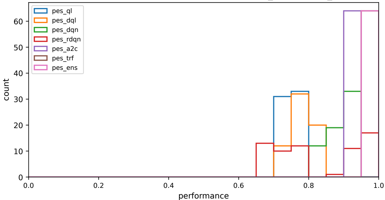
Per-sequence performance distribution -- sev_extrapolate_high
