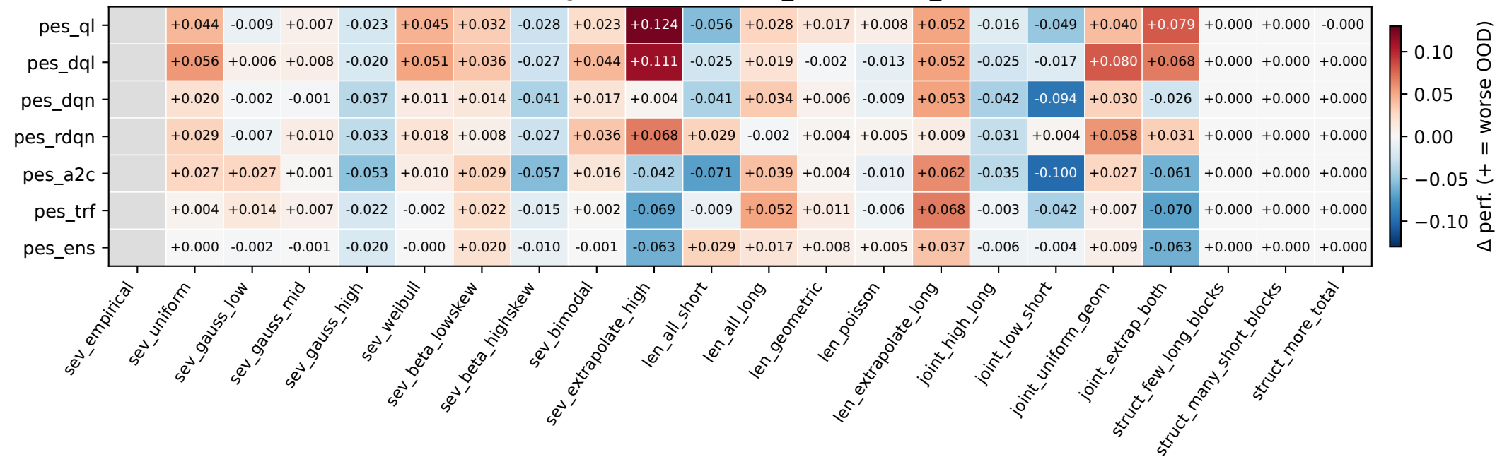
OOD degradation: baseline_mean – cell_mean
